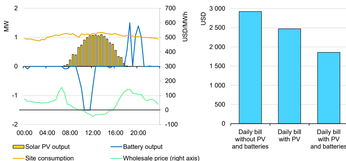
Site production, storage and consumption (left) and daily bill (right) of a large commercial energy user in South Australia on a typical day in 2023
