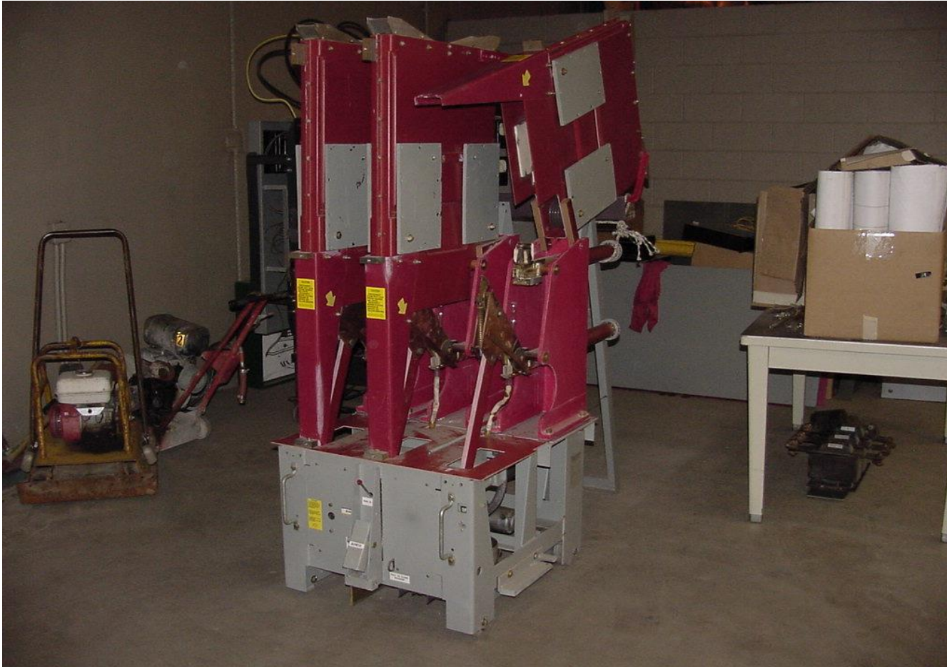
Air Magnetic Circuit Breaker
