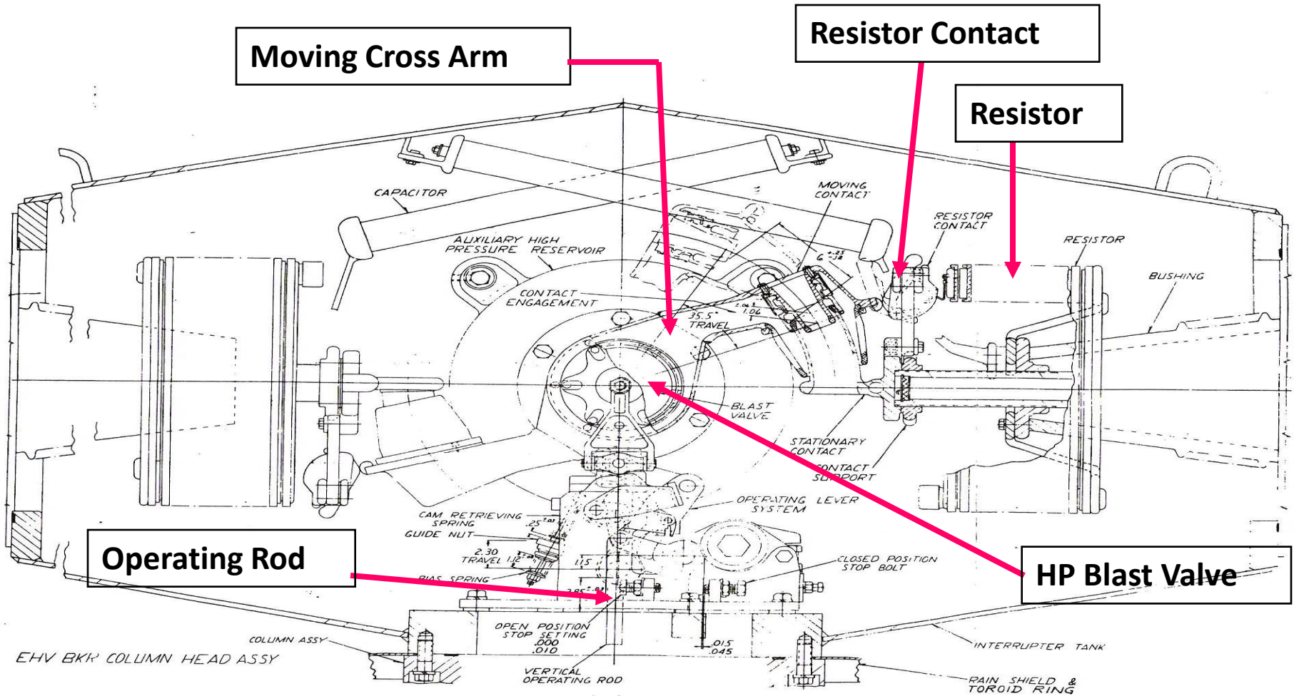
Side View of Gas Blast Breaker Interrupter Head
