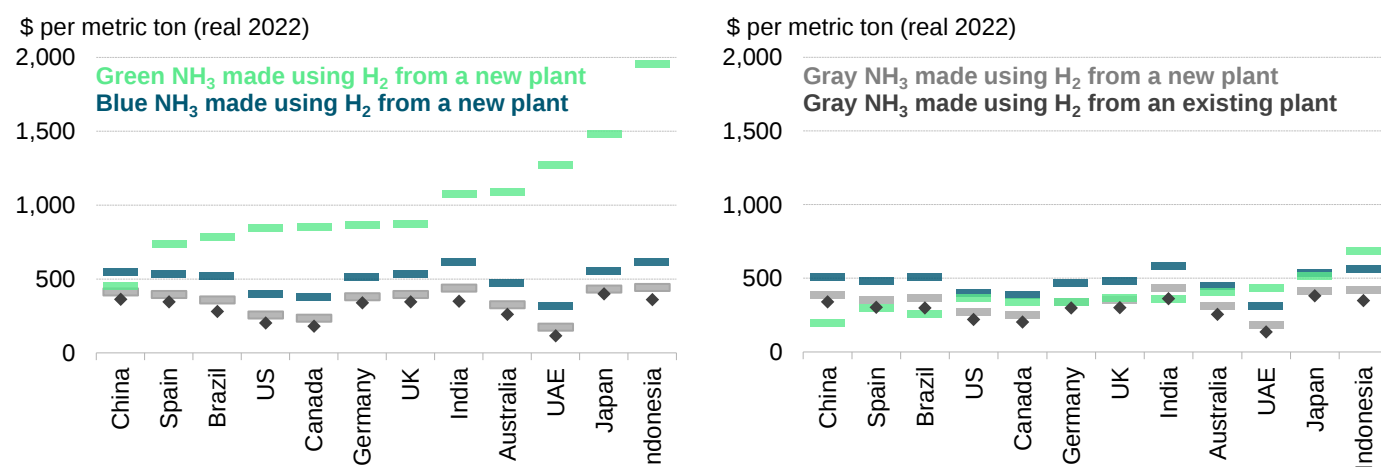
Figure 1: Cost of ammonia production in 2023 (left) and 2030 (right)
