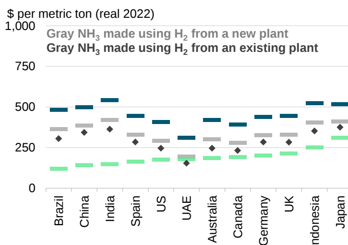
Figure 8: Cost of ammonia production in 2040
