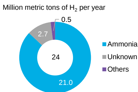
Figure 11: Planned hydrogen export capacity in end-product form (2022)
