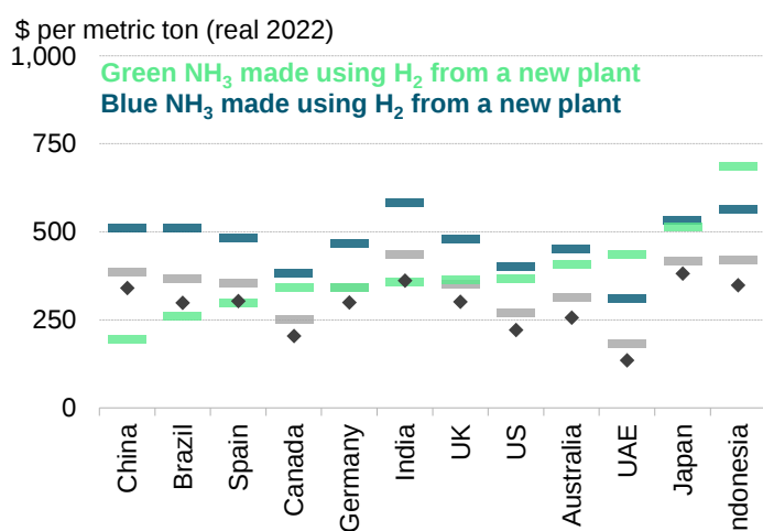
Figure 7: Cost of ammonia production in 2030
