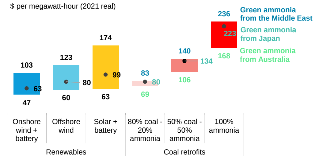
Figure 10: Comparison of levelized cost of electricity for different technologies in 2050
