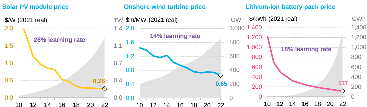
Figure 17: Price benchmark for solar modules, onshore wind turbines and battery packs, by year
