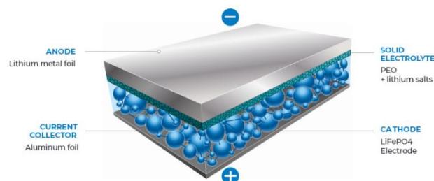
Figure 7. Blue Solutions' LMP ® battery [95].
