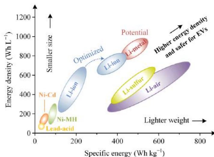
Figure 5. Specific energy and energy density of lithium-based batteries [34].
