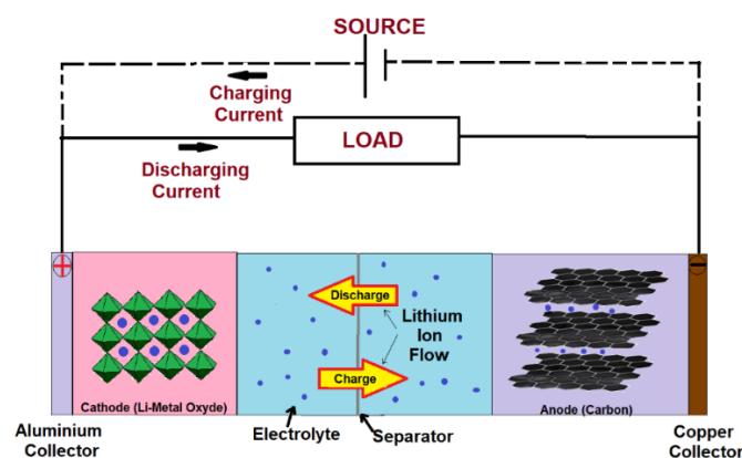
Figure 4. Schematic of the Lithium-Ion battery.
