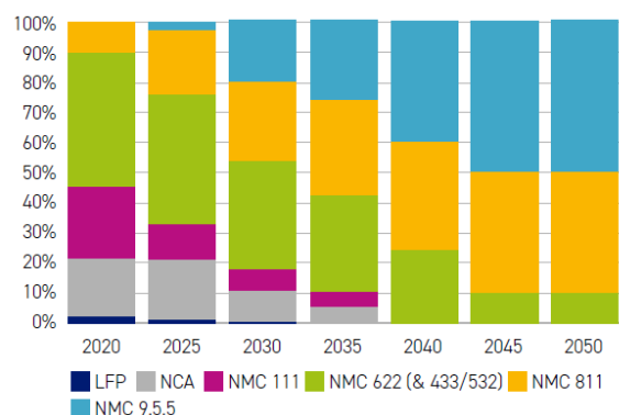
Figure 2. Different cathode types of EV battery chemistries from 2020 to 2050 [41].
