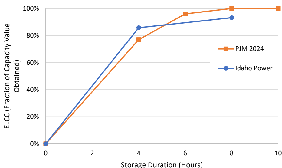
Figure 6. Annualized capacity value as a function of duration in PJM and Idaho Power using ELCC shows the potential for additional value beyond 4 hours.
