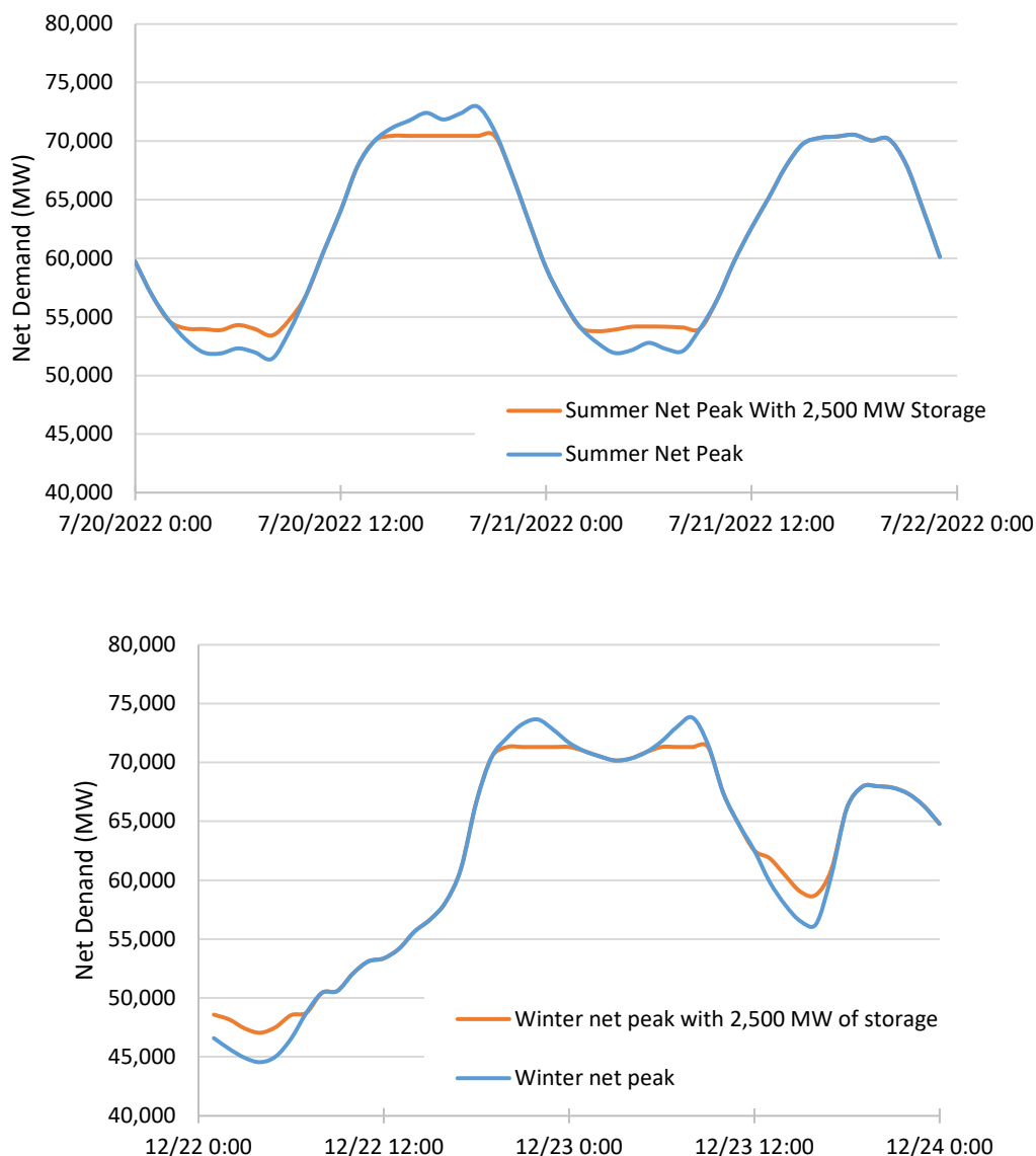
Figure 11. Addition of 2,500 MW of simulated storage in ERCOT widens net load peaks in the summer (top), but the wider peaks can be offset by additional solar. The impact of storage in the winter (bottom) is to widen the net peak mostly at night, which cannot be reduced with solar. This would require significantly more than 4 hours of duration to provide high capacity credit.
