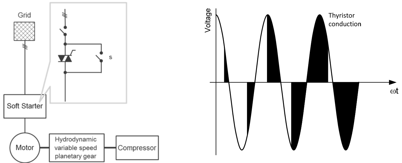
Figure 11 Motor with soft starter
