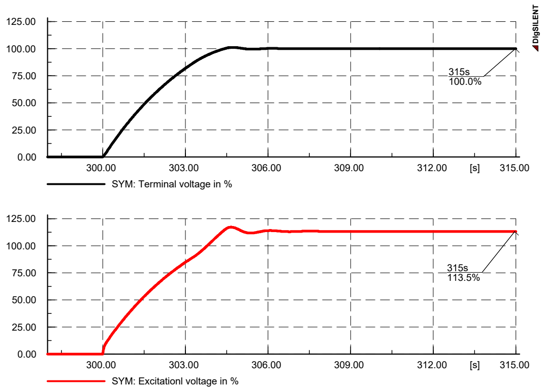
Figure 20 Switching on excitation
