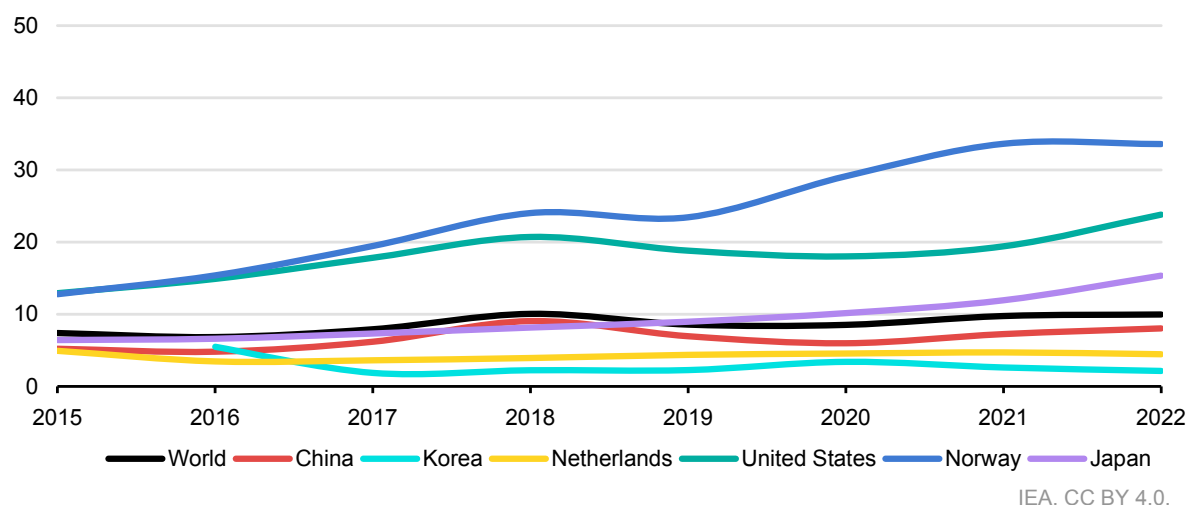
Figure 1.15 Electric light-duty vehicle per public charging point, 2010-2022
