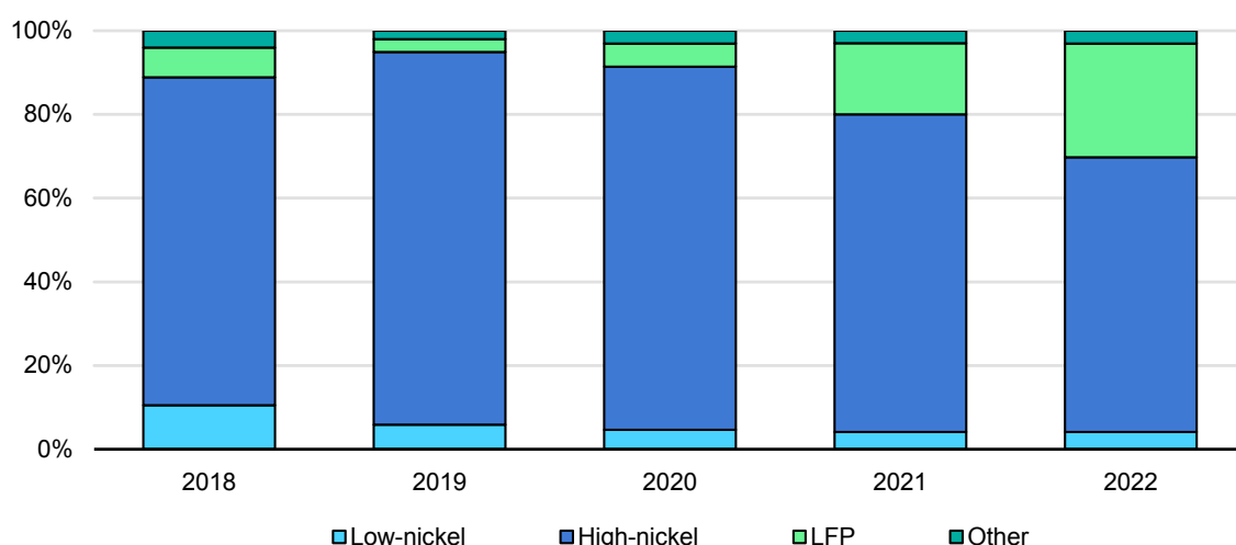
Figure 1.19 Electric light-duty vehicle battery capacity by chemistry, 2018-2022
