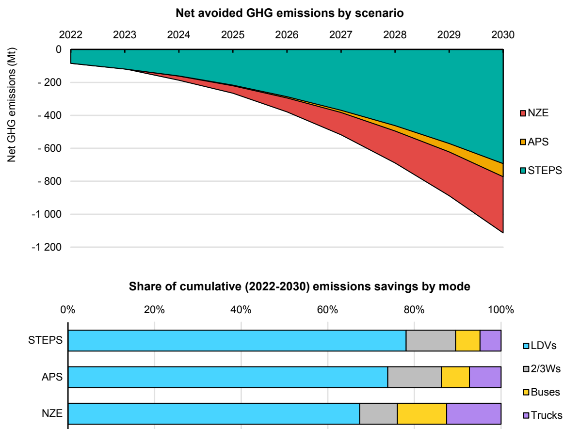
Figure 3.15. Net avoided greenhouse gas emissions from EV deployment and share of avoided emissions by mode, 2022-2030
