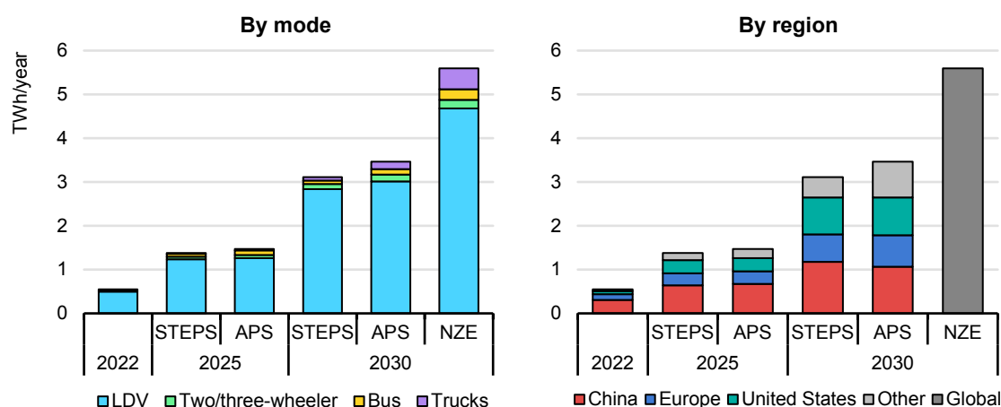
Figure 3.7. Projected battery demand by mode and region, 2022-2030
