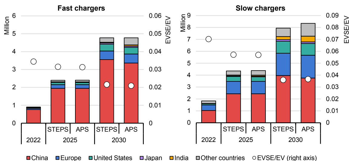
Figure 3.10. Number of public light-duty vehicle chargers installed by region, 2022-2030
