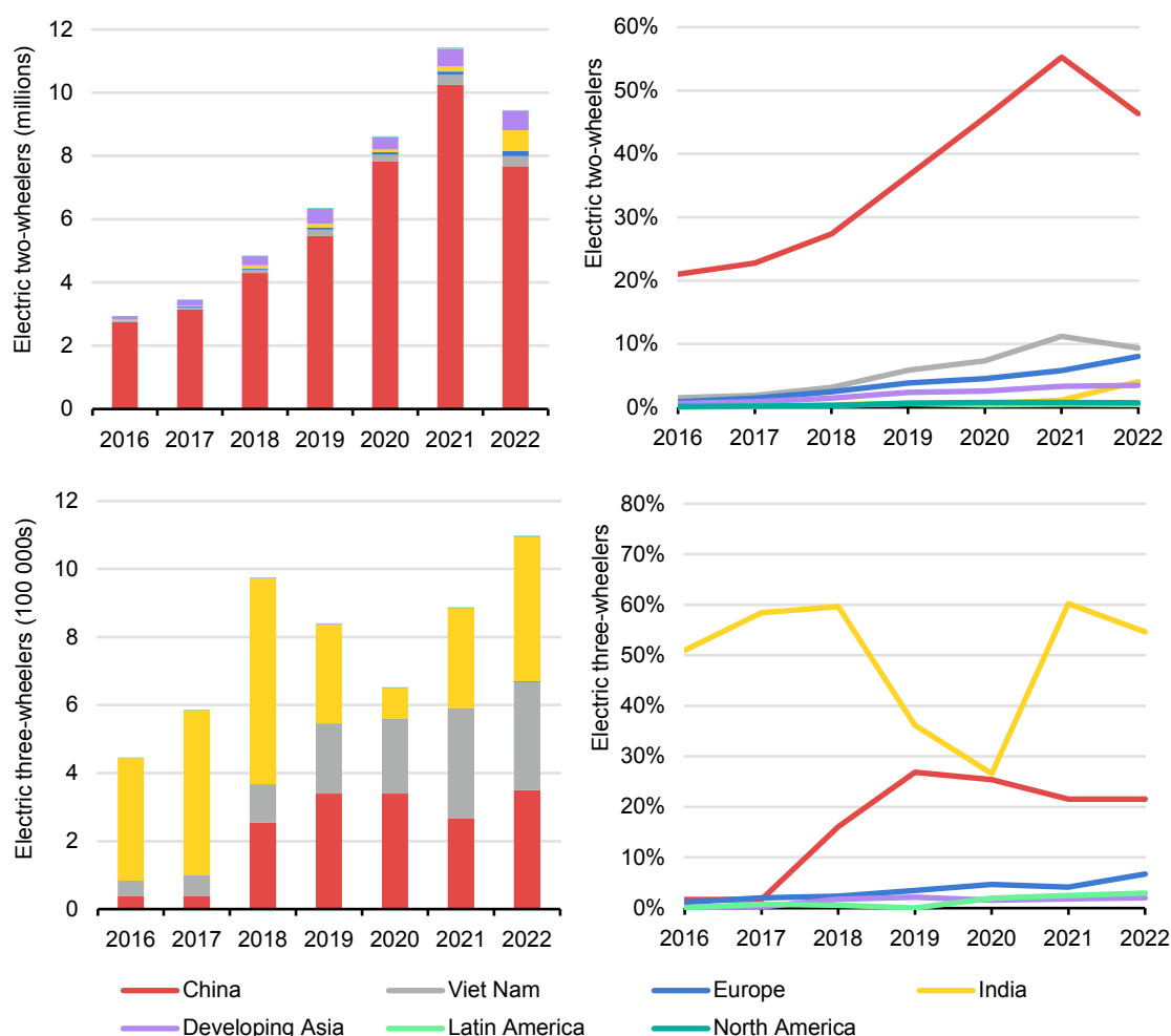
Figure 1.10 Electric two- and three-wheeler sales and sales share by region, 2016-2022
