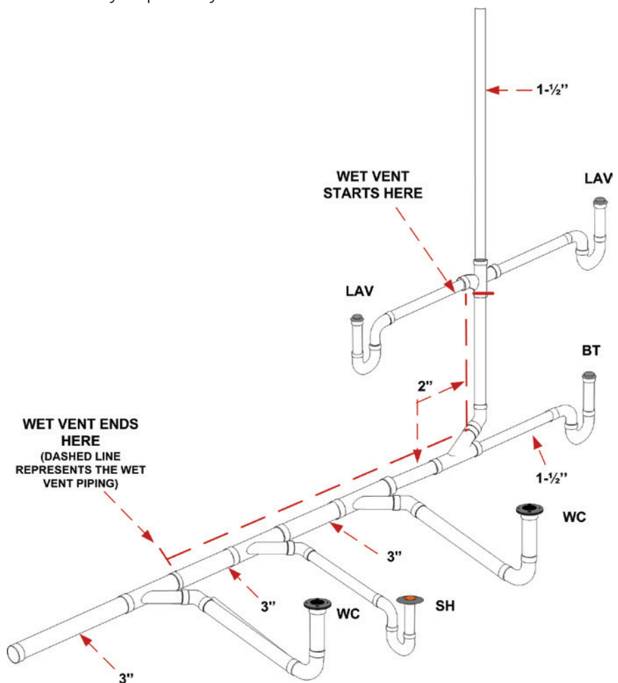
Figure 8: Horizontal Wet Venting Illustration
