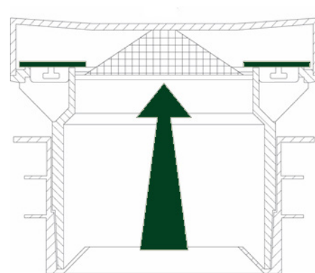
Figure 3: Air admittance valve closes and seals under zero or positive pressures
