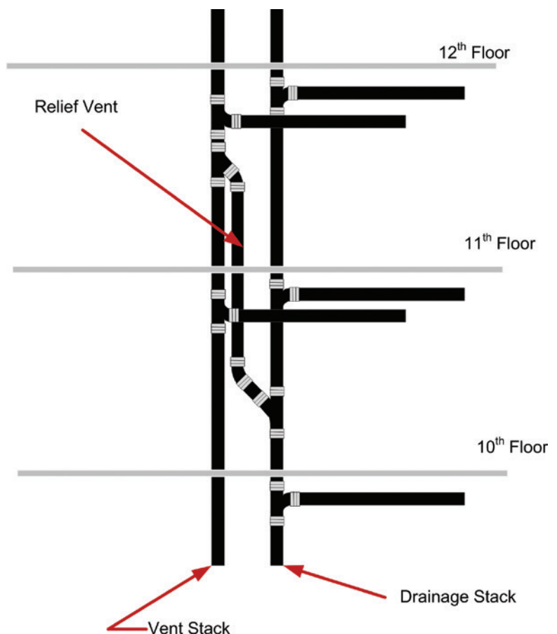
The graphic illustrates a relief vent connection.
