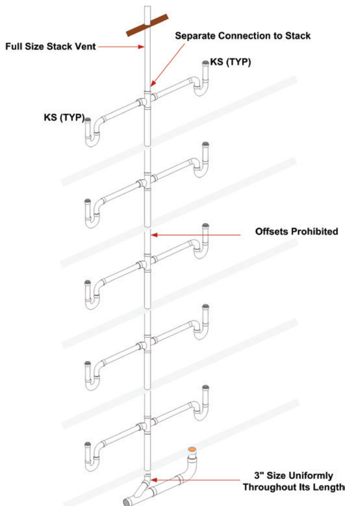
Waste Stack Vent
