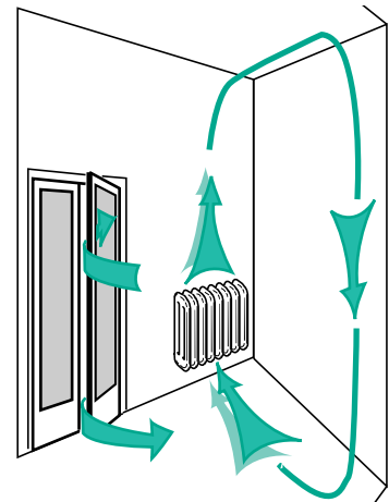
fig. 6: convection currents.
