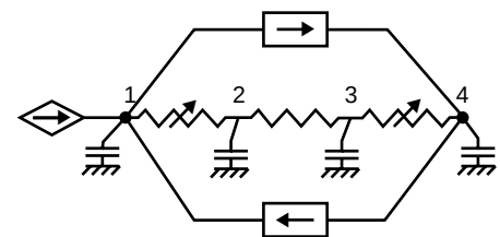
fig. 8: Correspondence between thermal and electrical quantities.
