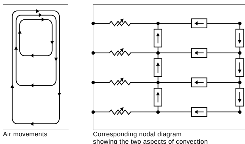
fig. 10: mass and thermal modelling of convection.
