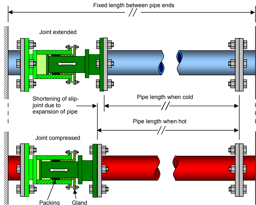
Figure 4.6: Action of Slip-type Expansion Joint
