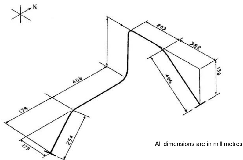
Figure 5.5: Piping Isometric—Linear Dimensions Only
