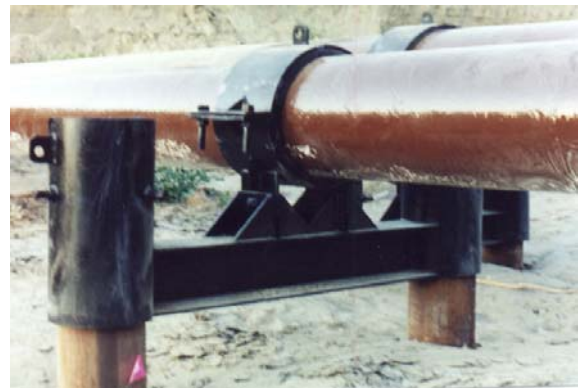
Figure 2.12: Clamped Support
