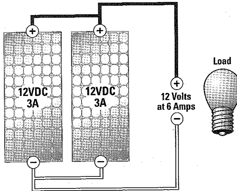
Figure 2-3 PV MODULES IN PARALLEL
