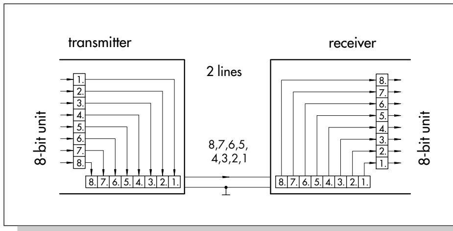
Fig. 9: Serial data transmission
