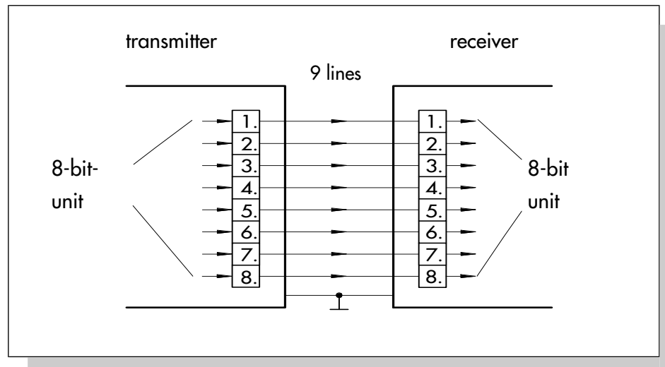
Fig. 8: Parallel data transmission
