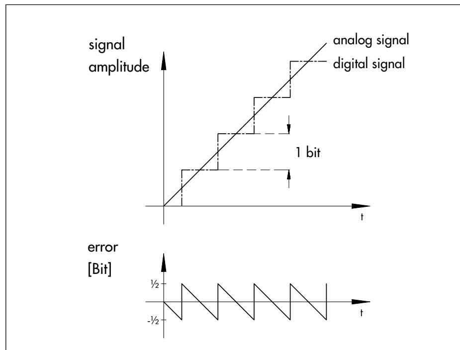
Fig. 3: Quantization error caused by reduced discretization and sampling rate
