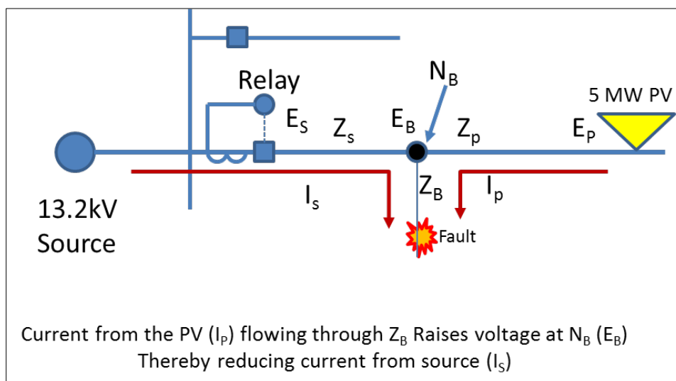
Figure 2.11. Reduction in fault current through substation relay because of PV
