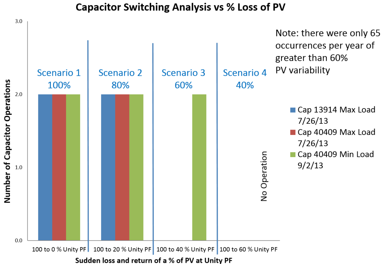
Figure 3.14. Porterville example study results—capacitor switching compared to percentage loss of PV
