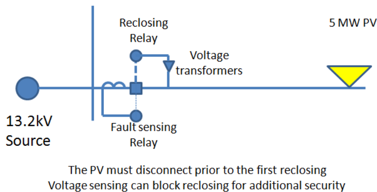
Figure 2.14. Reclosing out of synchronism
