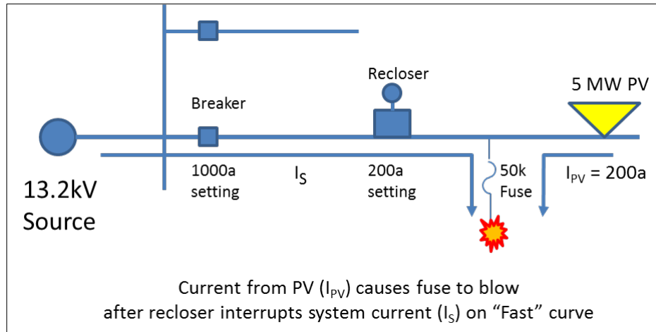
Figure 2.13. Illustration of nuisance fuse-blowing caused by large PV penetration
