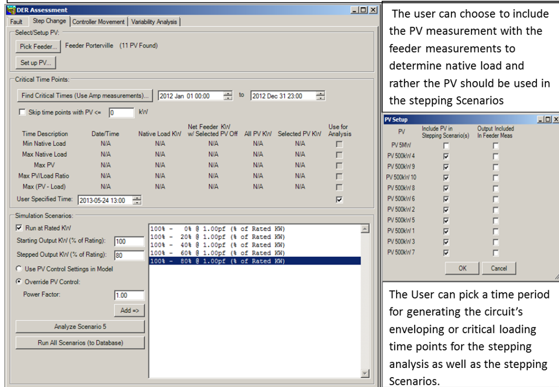
Figure 3.9. DEW's DER automated assessment application dialog
