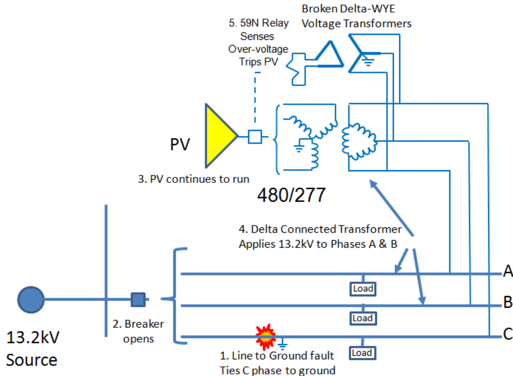
Figure 2.12. PV may cause line-to-ground overvoltage
