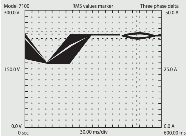
Example of recording of a voltage dip
