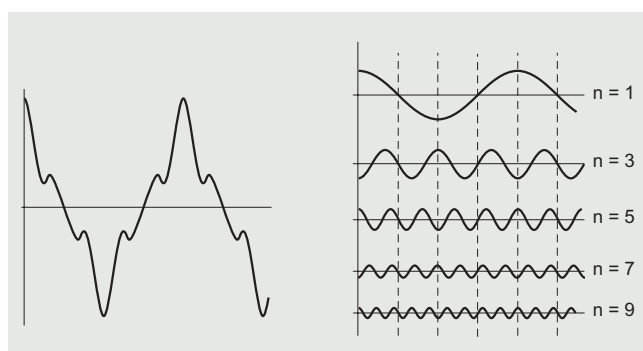
^ Signal distorted by the presence of harmonics, particularly order 3 and 5 which are typical in commercial environments (electrical power supplies, computers)
