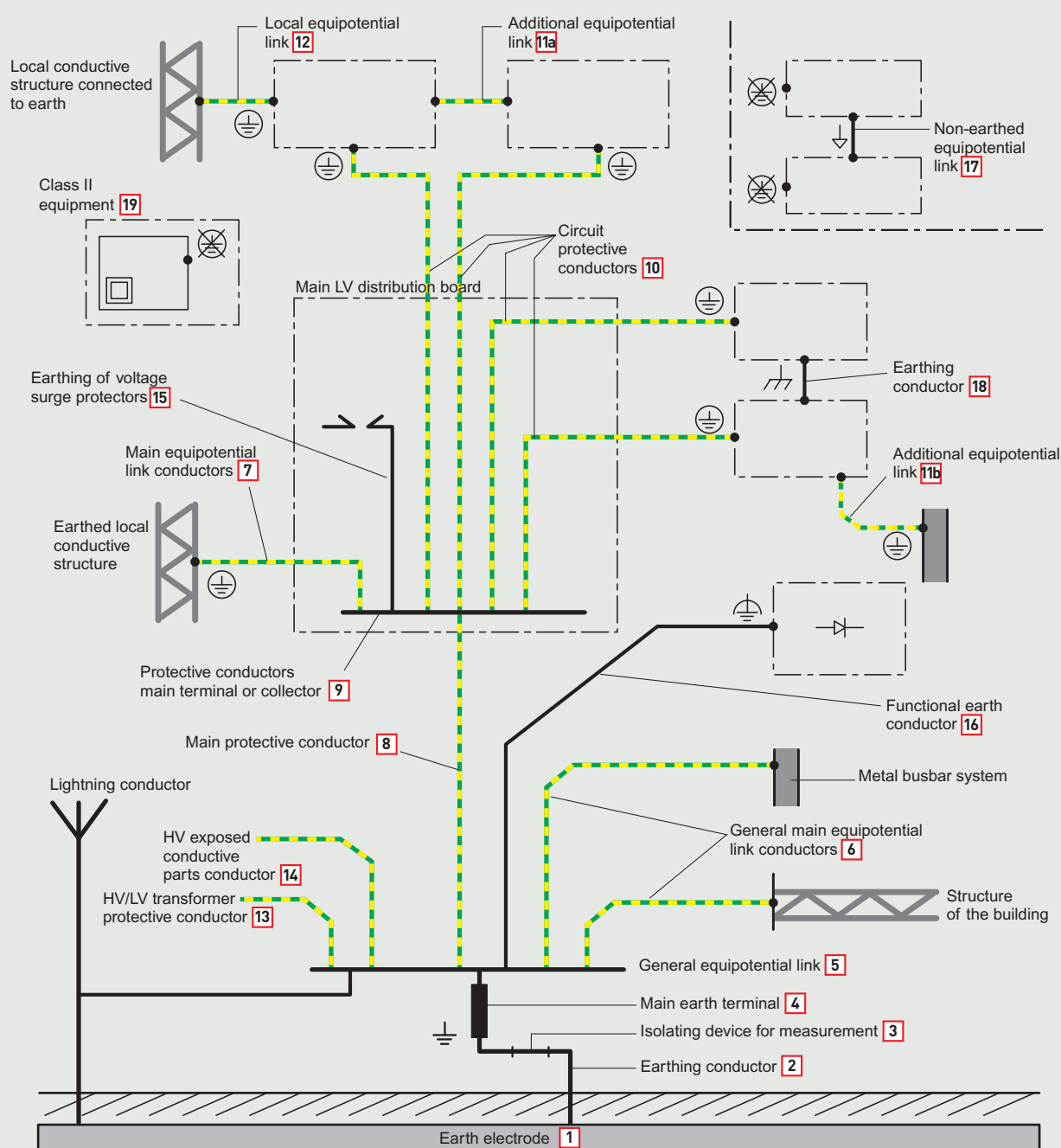
Diagram of the protection system (see definitions on the following pages)
