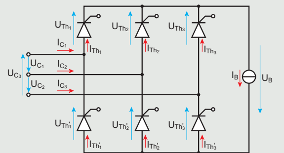
Thyristor bridge rectifier at the input of a conventional AC/DC converter
