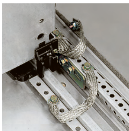
^ Earthing conductors consisting of braids (30 mm 2 )
