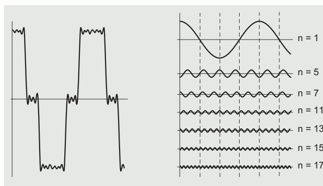
^ Signal distorted by the presence of high harmonics orders, particularly orders 5 and 7 (even 11 and 13), typical of industrial environments (frequency controls for example)
