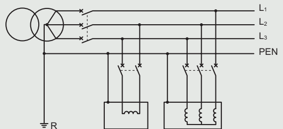
TN-C system
