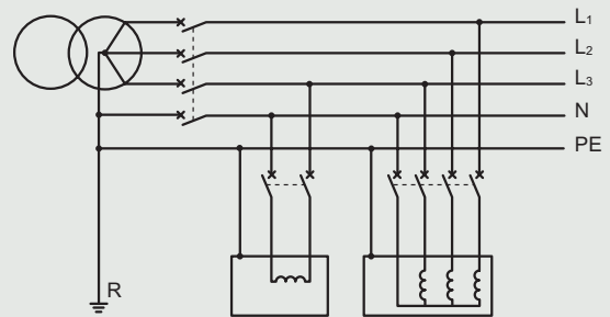
TN-S system
