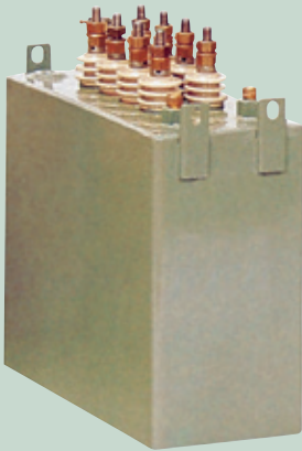
Water-cooled capacitor for medium frequency induction furnaces
