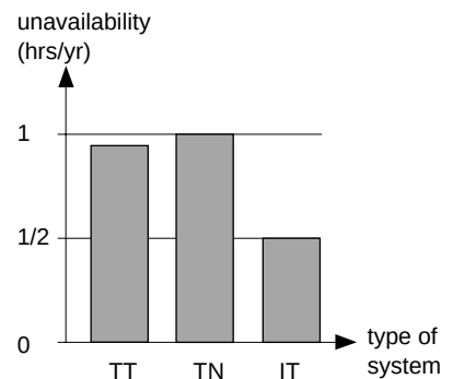
c) unavailability on a feeder as a function of the system earthing arrangement
