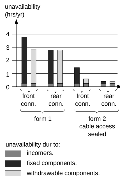
fig. 12: unavailability times depend on switchboard technology and particularly on its connection type (the chart corresponds to the diagram in figure 10).
