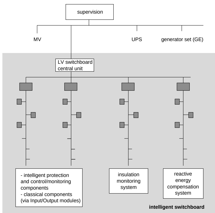
fig. 18: general diagram showing control and monitoring of an electrical installation and its links (BUS) supervision.
