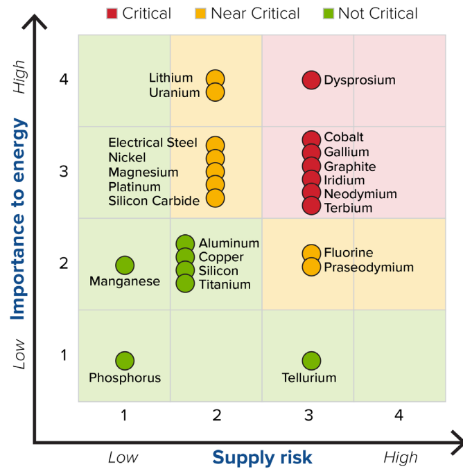
Figure ES.1. Short-term (2020–2025) criticality matrix
