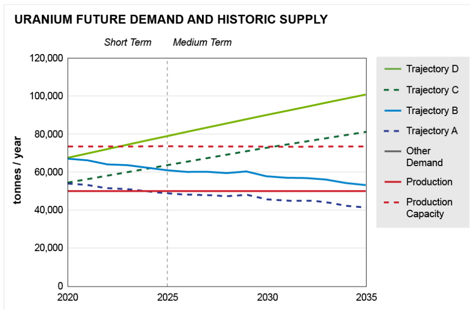
Figure 4.41. Uranium demand trajectories, current production, and production capacity.
