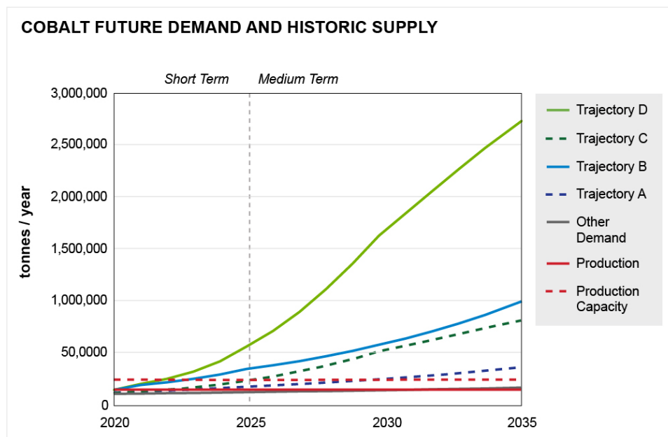
Figure 4.20. Cobalt demand trajectories, current production, and production capacity.
