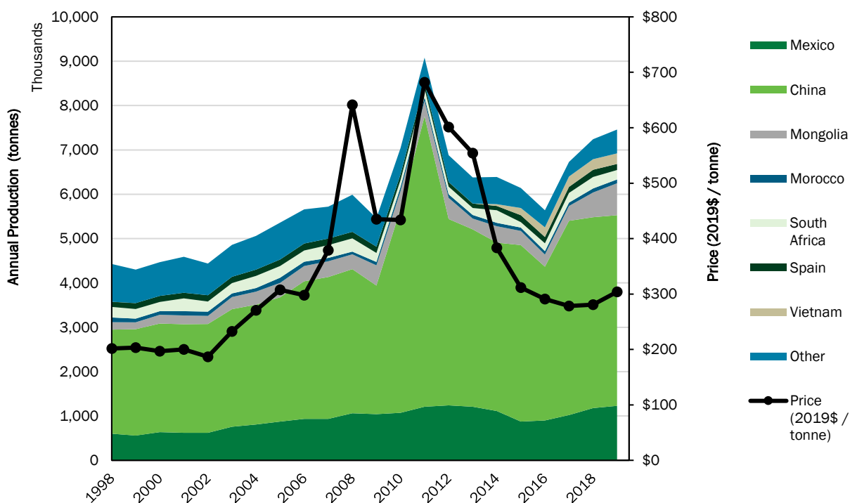
Fluorspar Production and Prices
