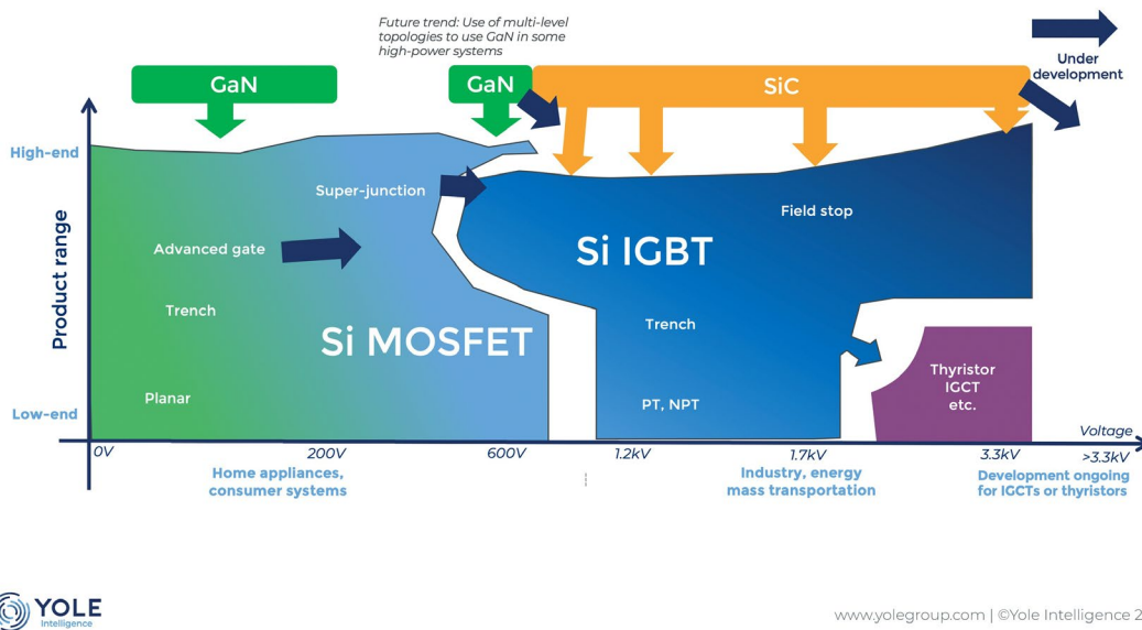
Figure 2.3. Performance of Si, SiC, and GaN power electronics. Top: based on switching power and operating frequency; bottom: based on voltage (Rosina & Villamor, 2022).
