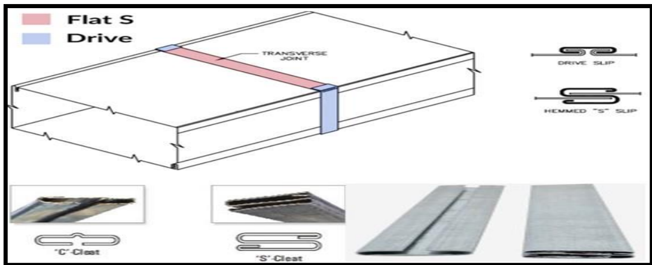
Slip and Drive Fixing and Ducting Connection
