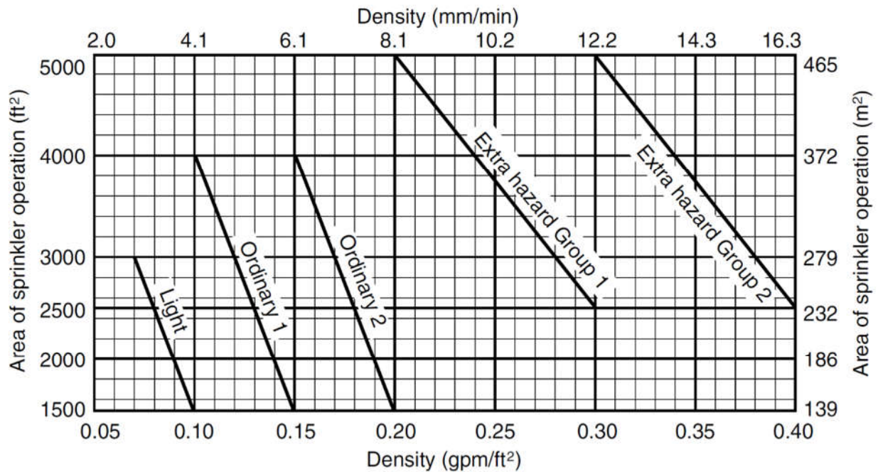
FIGURE 11.2.3.1.1 Density/Area Curves.
