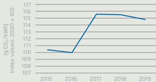
CO 2 intensity of power
