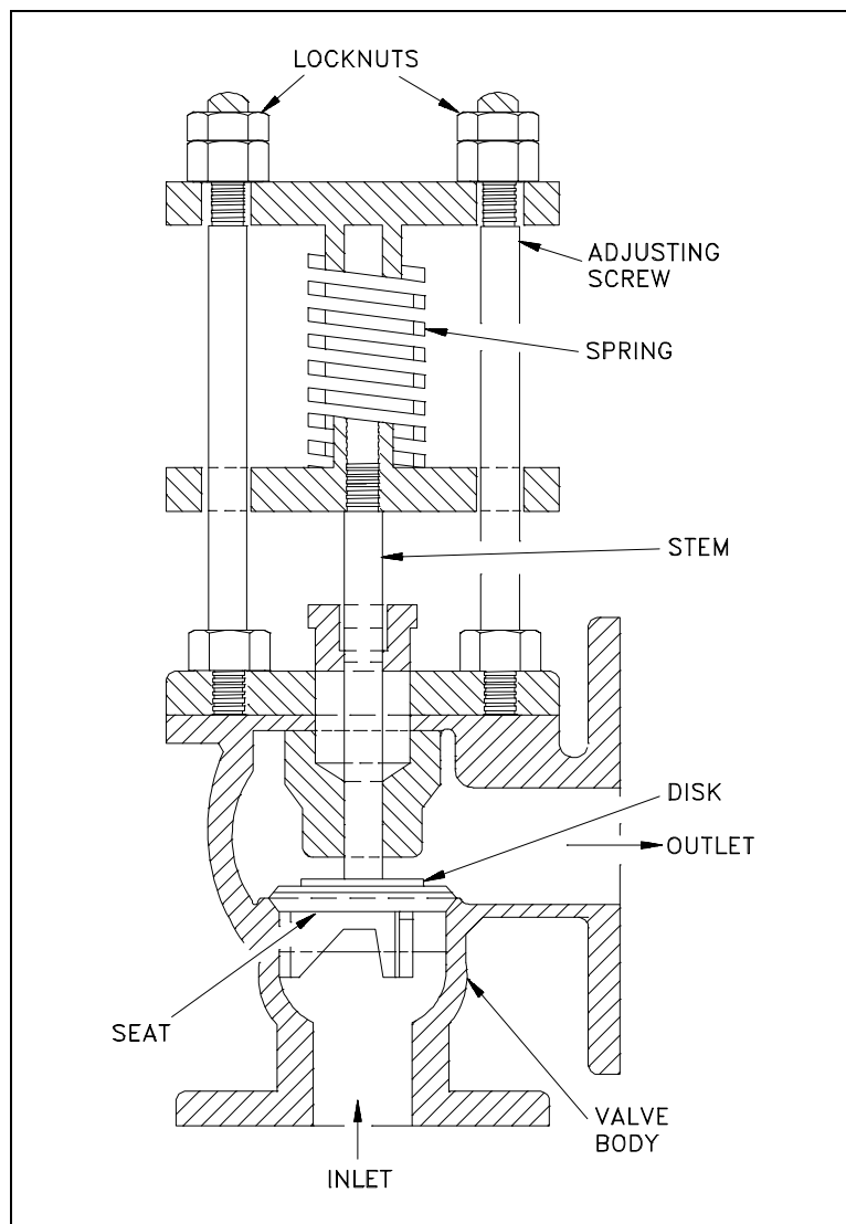
Figure 28 Relief Valve
