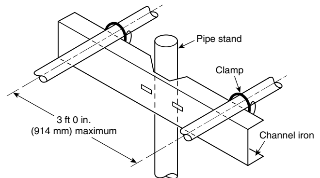
FIGURE A.6.3.2.2.8(d) Multiple Pipes Supported by One Pipe Stand.
