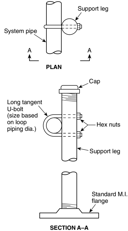
FIGURE A.6.3.2.2.8(c) Acceptable Attachment for Pipe to Support Legs — Example 2.
