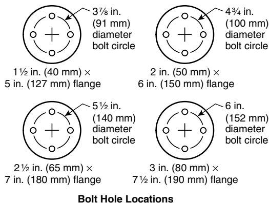
FIGURE A.6.3.2.2.7 Support Leg Footings.
