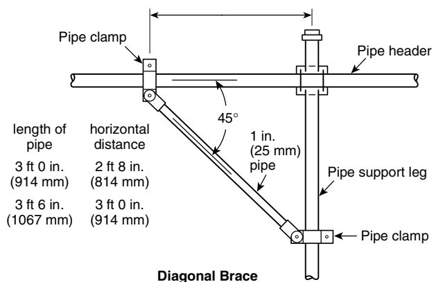
FIGURE A.6.3.2.2.2 Typical Arrangement of Support Legs for Pipe Stands.
