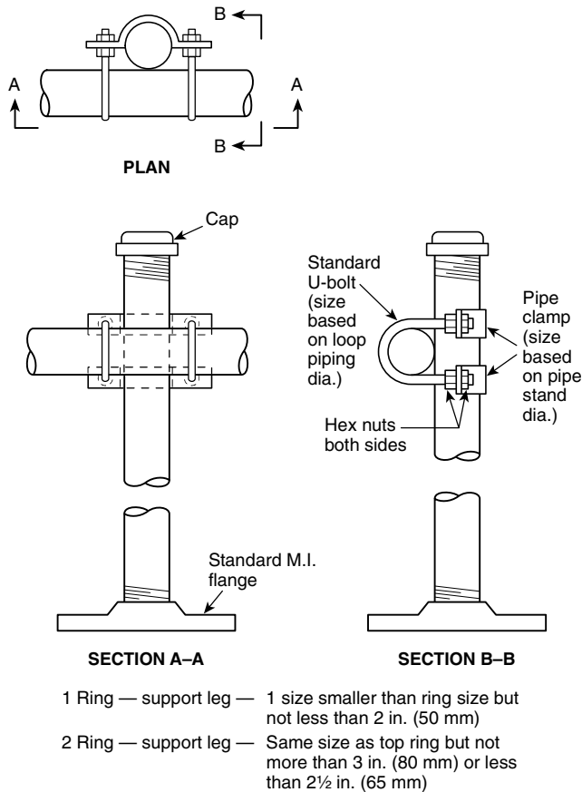
FIGURE A.6.3.2.2.8(b) Acceptable Attachment for Pipe to Support Legs — Example 1.
