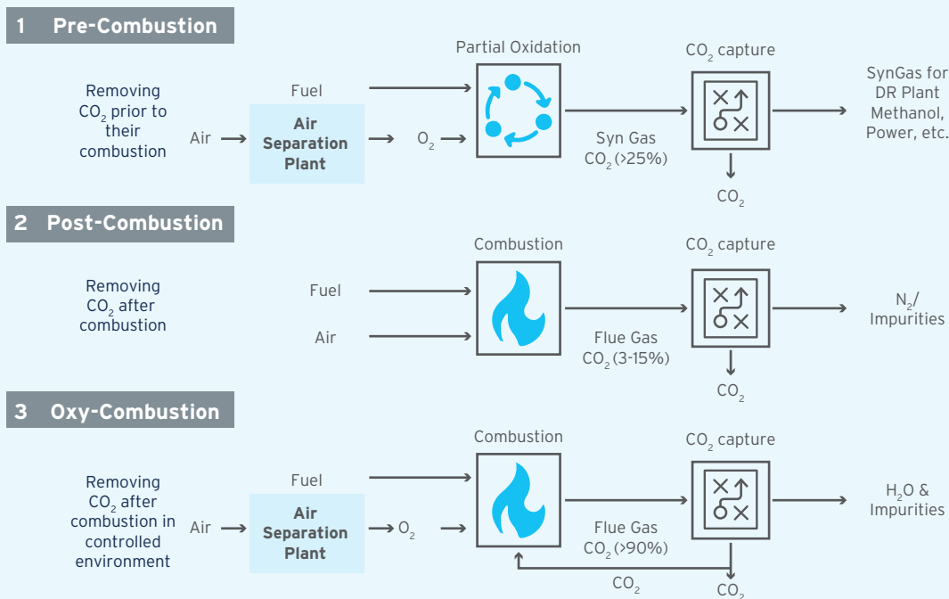
Figure 3-1: Scheme of Post-combustion, Pre-combustion & Oxy-fuel combustion
