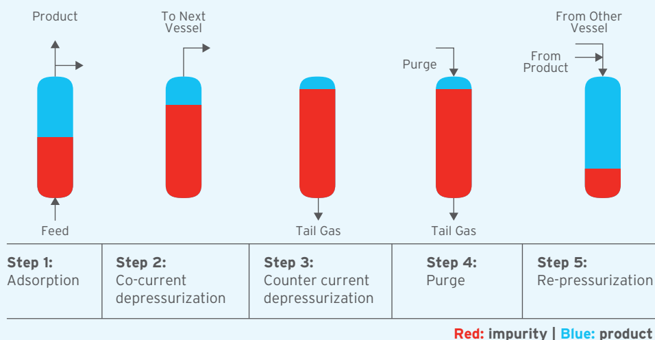
Figure 3-15: Five-step Pressure-swing Cycle of UOP's Polybed™ PSA Systems
