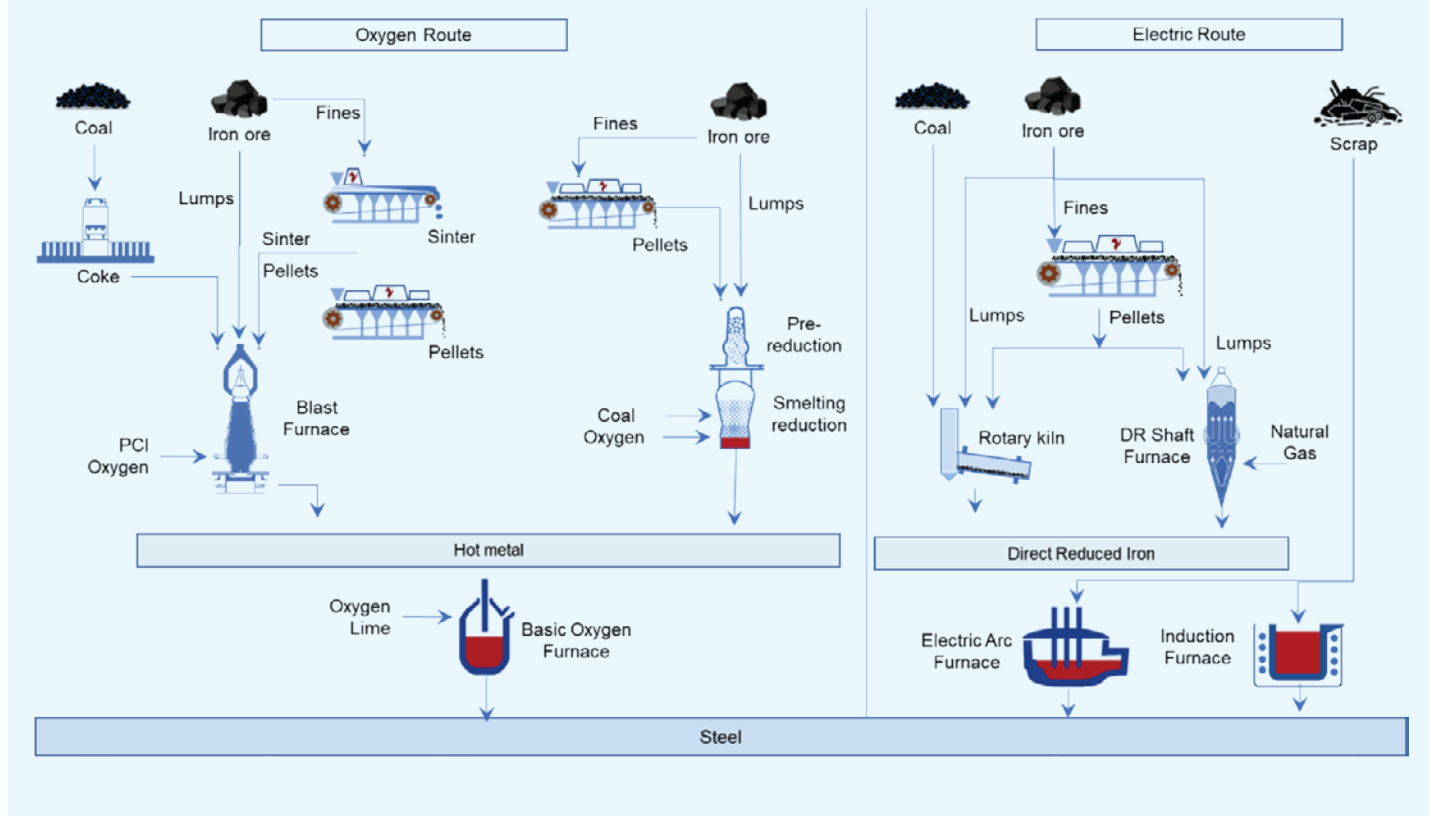
Figure 2-13: Various Iron and Steel Making Routes in India
