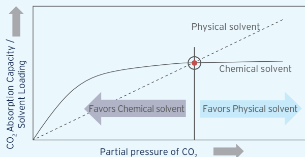
Figure 3-4: Schematic Representation of CO 2 Absorption Capacity of Chemical and Physical Solvents as a Function of the Partial Pressure of CO 2
