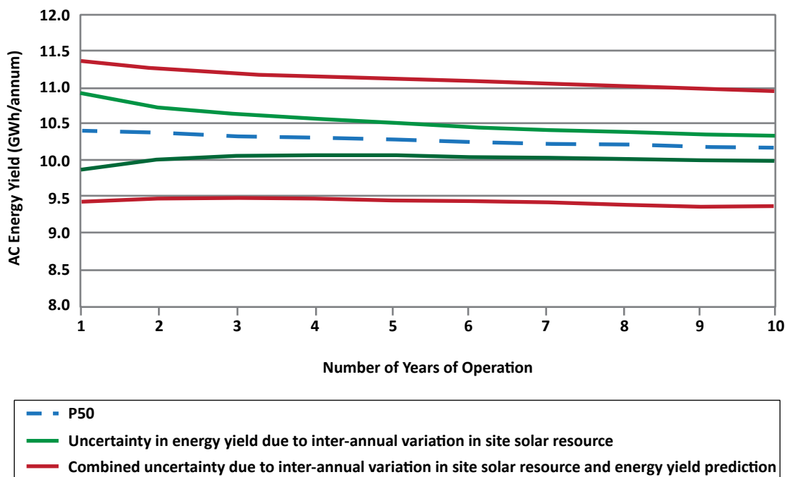
Figure 15: Uncertainty in Energy Yield Prediction
