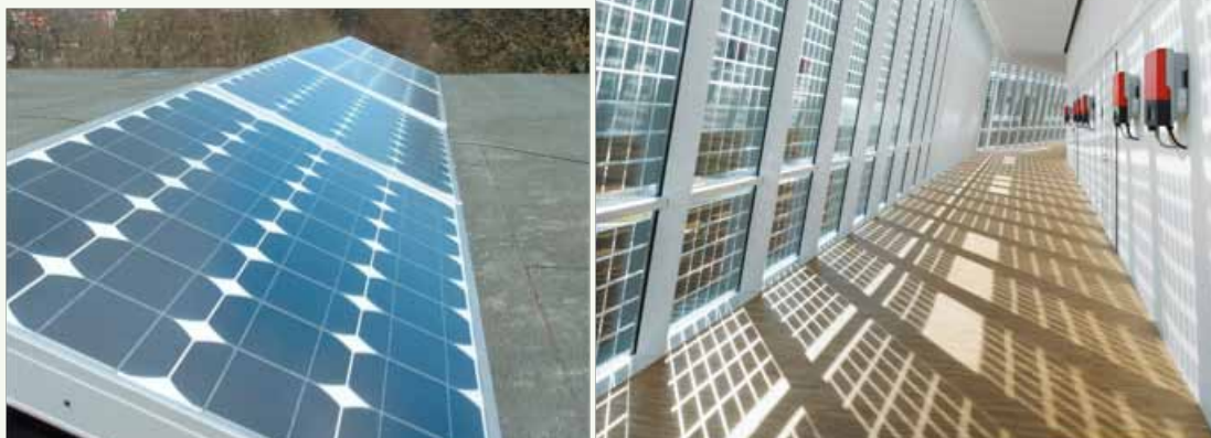
Figure 35: BAPV (Left) and BIPV (Right) Systems
