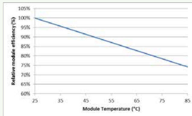
Figure 36: Reduction in Module Efficiency with Average Temperature Coefficient
