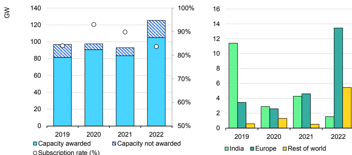
Global renewable energy auction results (left) and volumes of unawarded auction capacity by region (right)
