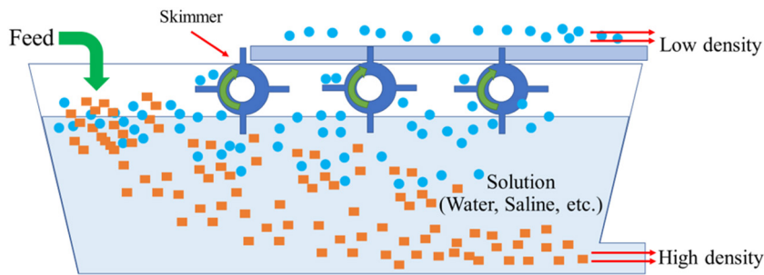
Figure 6.24 Sink-float separation.
