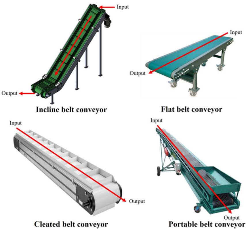
Figure 6.10 Conveyor belt used for lightweight materials (Source: modified from https://www.beidoou.com/construction/belt-conveyor-types.html ).
