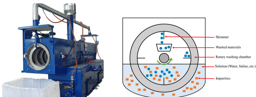
Figure 6.20 Rotary washer (Source: Rotajet Systems Ltd., 2020).
