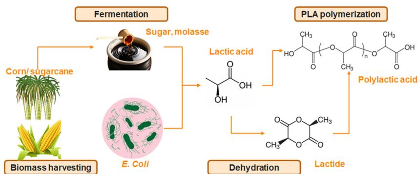
Figure 10.12 Schematic of PLA fabrication process.
