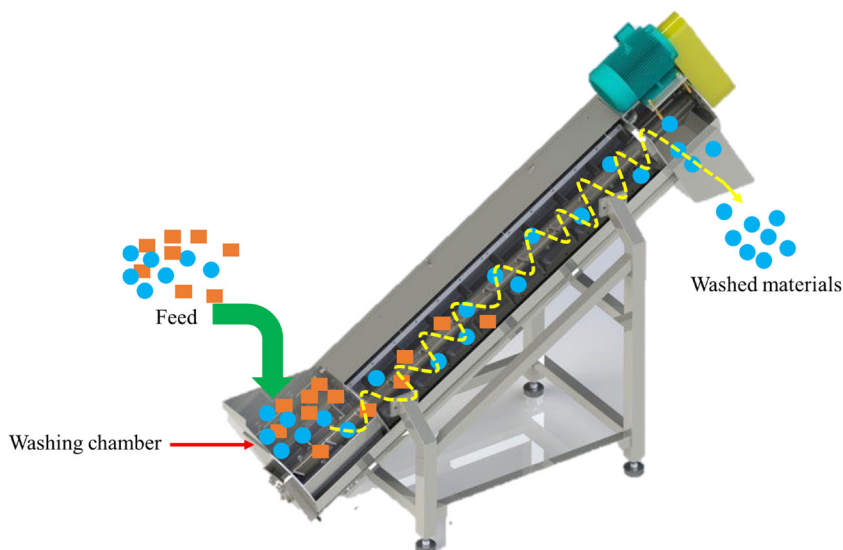
Figure 6.21 Friction washer (Source: https://www.ldmachinery.com/index.php?r=article/Content/index&content_id=28 ).
