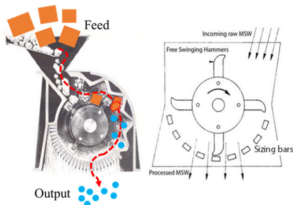
Figure 6.17 Hammer mill shredder (Source: Fitzgerald & Themelis, 2009).
