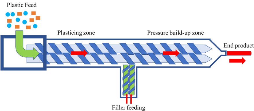
Figure 6.31 Process zones of a twin-screw extruder (Source: Bonten, 2019).
