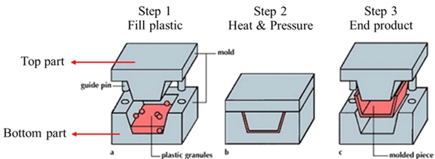
Figure 6.33 Mold compression (Source: https://kids.britannica.com/students/assembly/view/53835 )
