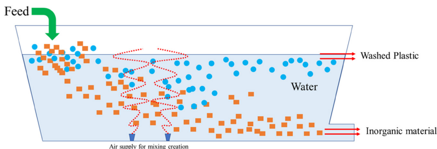
Figure 6.19 Floating washer.
