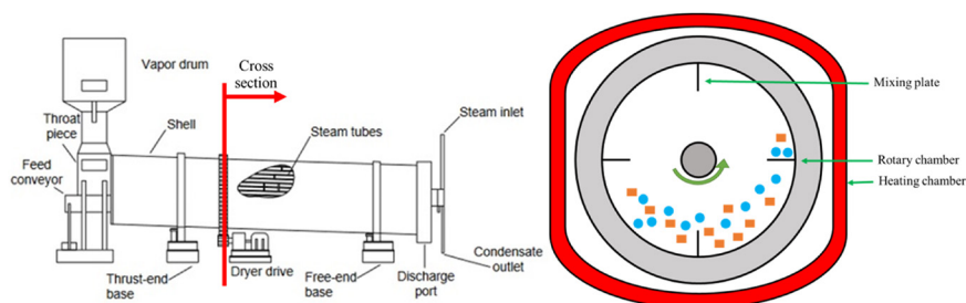
Figure 6.23 Rotary dryers (Source: Mujumdar, 1995).
