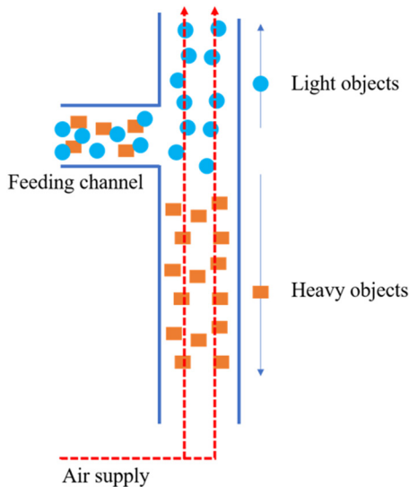
Figure 6.13 Schematic diagram of air classifier.
