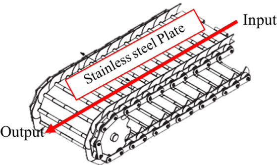
Figure 6.11 Hinged steel belts for heavy material (Source: OETIKER International; http://dktransportbaand.dk/upload_dir/pics/ALLERT_Hinged_Steel_Belts.pdf ).
