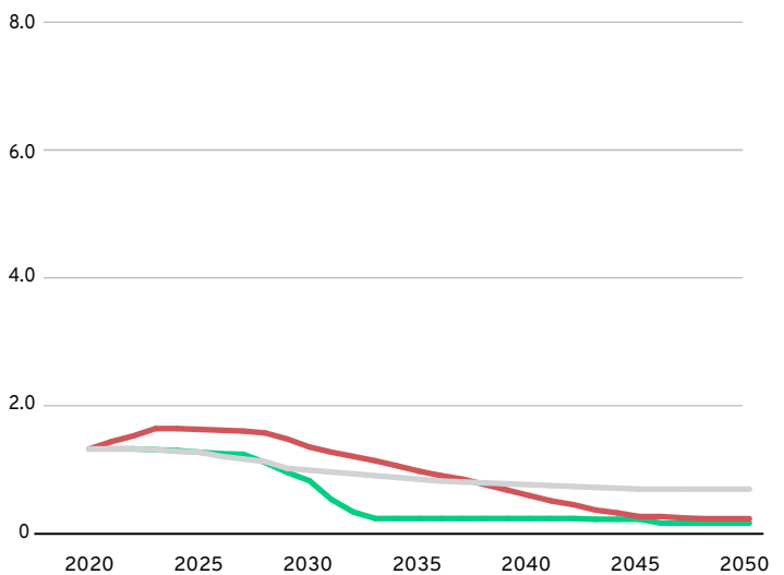
Coal consumption in ammonia production, EJ/year
