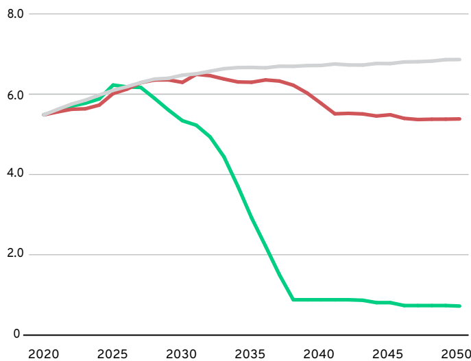
Natural gas consumption in ammonia production, EJ/year
