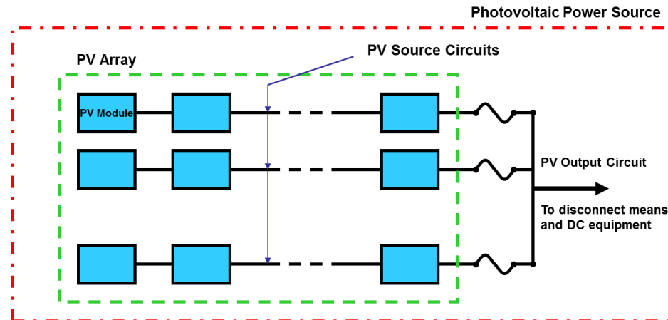
Figure 48: PV Power Sources Comprise PV Source and Output Circuits
