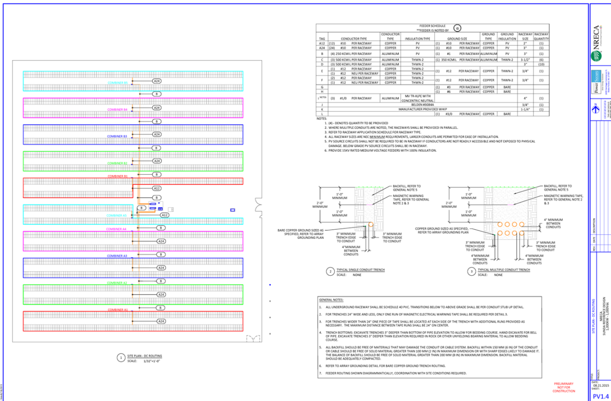
Figure 50: DC Circuit Layout for SUNDA 1-MW Reference Design
