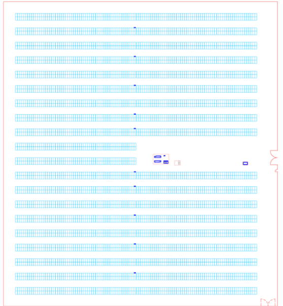
Figure 2: Overview of the SUNDA 1-MW Reference Design
