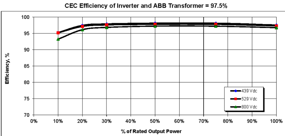
Figure 37: Inverter Efficiency Curves Show Power Conversion Efficiencies over a Range of Power and Voltage Levels (Conext Core XC-540-NA)
