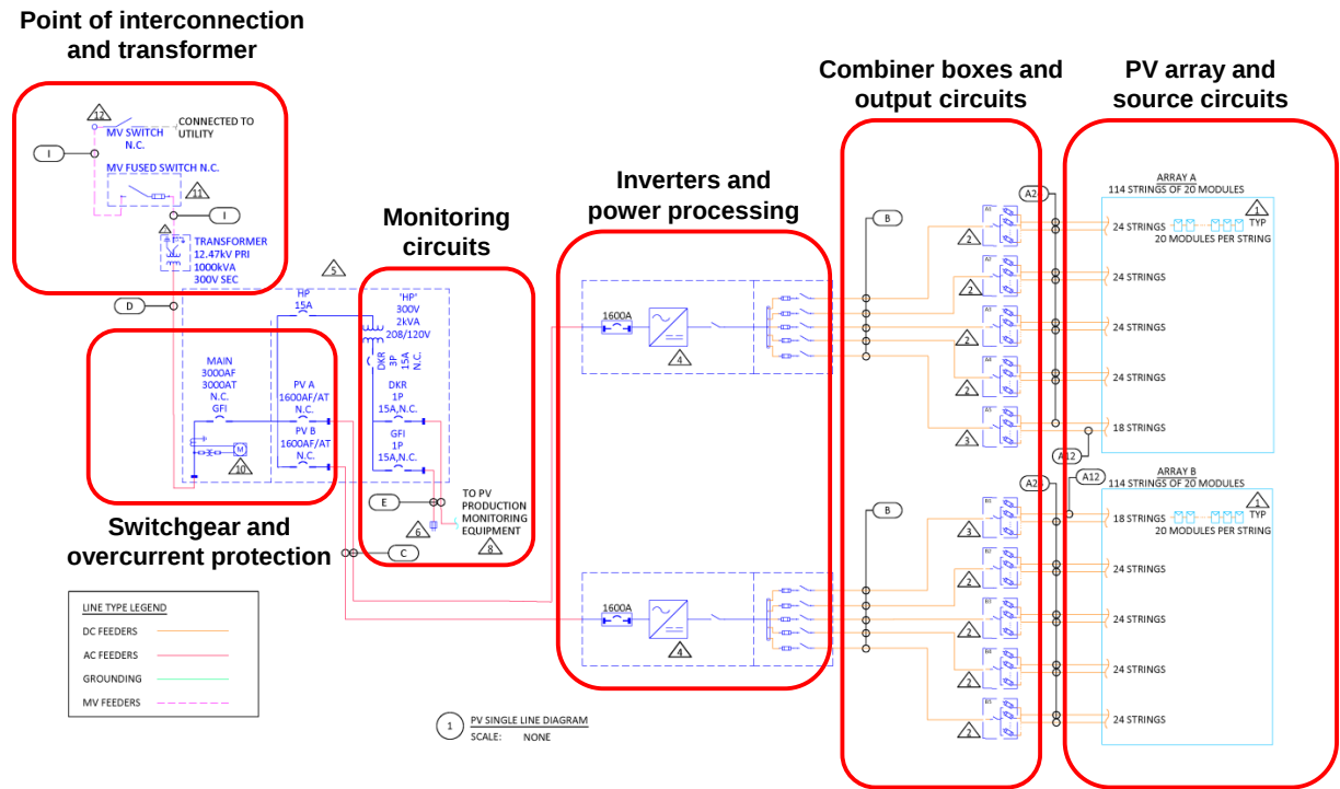
Figure 11: SUNDA 1-MW Reference Design
