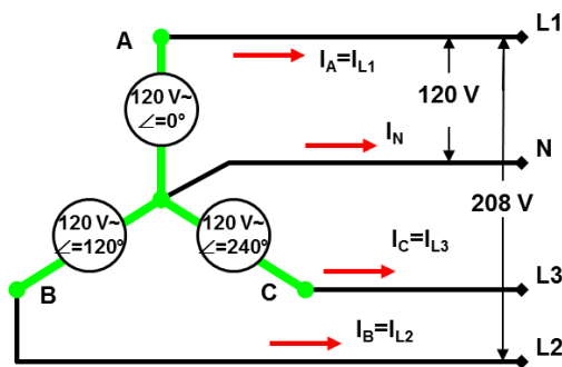
4-Wire, 120/208 V - Wye “Y”
