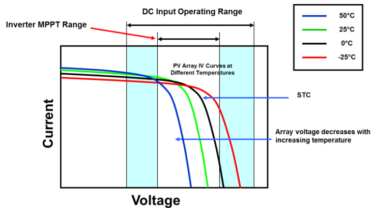
Figure 31: String Sizing Evaluates PV Array Voltage Compatibility with Inverter Input Requirements
