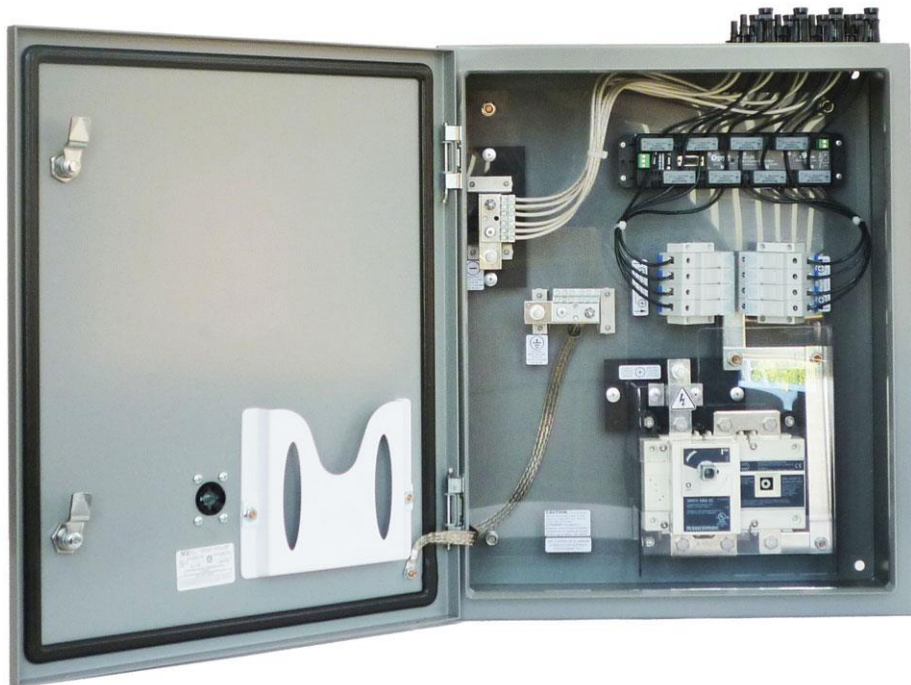
Figure 52: Combiner Box (courtesy of Solar Professional Magazine)
