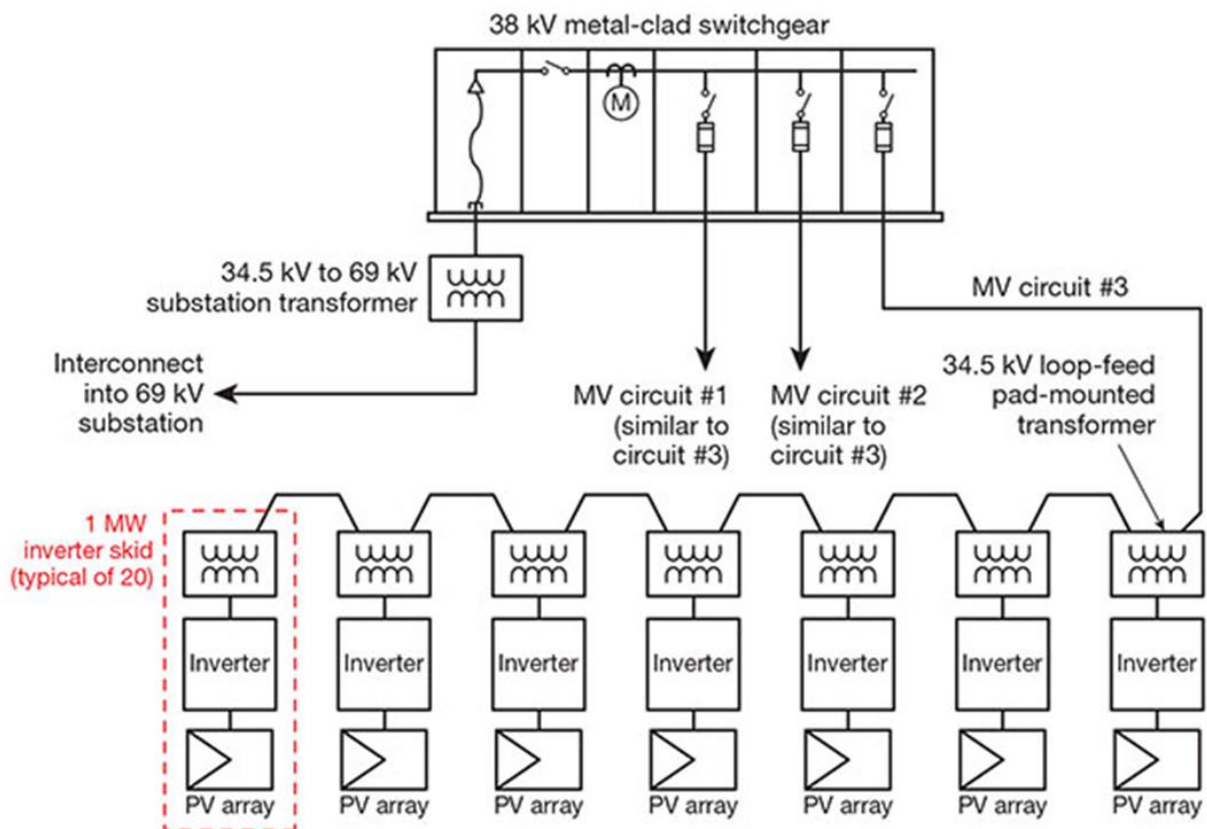
Figure 65: AC Collection Systems for Large Utility-Scale PV System
