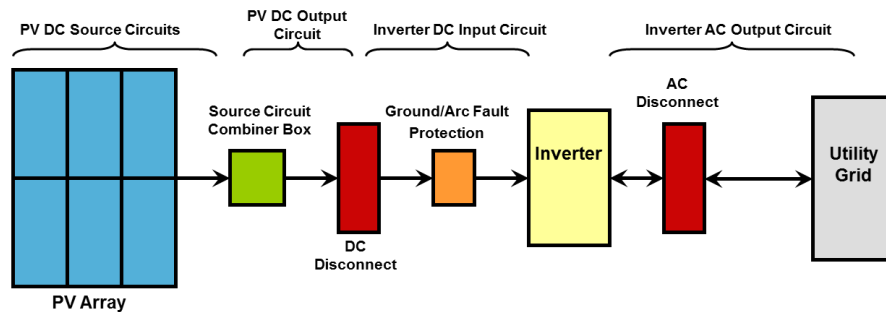
Figure 49: Interactive PV Systems Comprise Specific DC and AC Circuits
