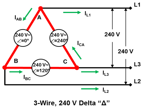
Figure 30: Delta Configurations Are Commonly Used for Commercial Services
