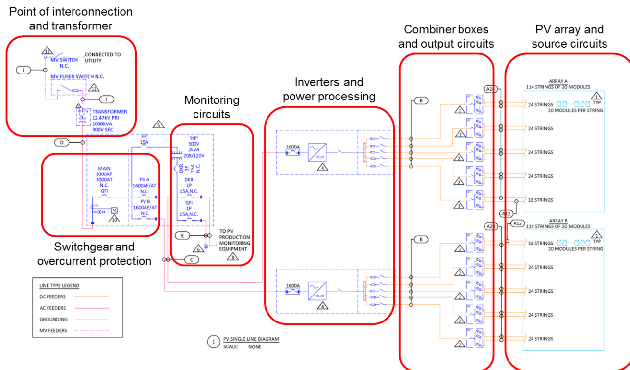
Figure 47: Single-Line Diagram for the SUNDA 1-MW Design
