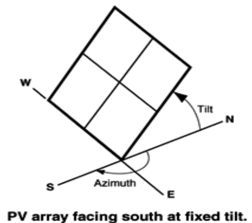
Figure 5: Tilt and Azimuth (image courtesy of NREL)
