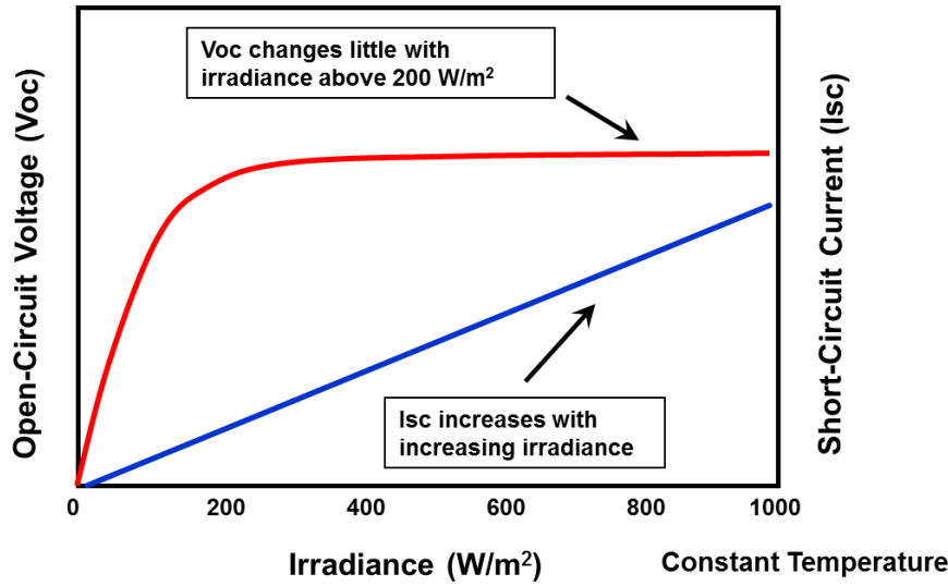
Figure 22: Open-Circuit Voltage Increases at Low Irradiance Levels, then Remains Relatively Constant as Irradiance Increases
