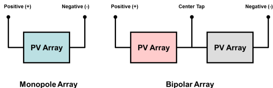
Figure 28: PV Arrays Can Be Configured as Monopole or Bipolar Arrays, Depending on Inverter Requirements
