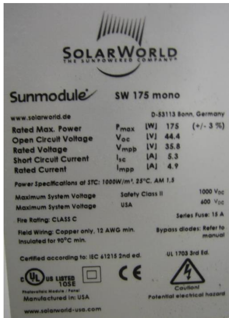
Figure 20: PV Module Labels Contain Important Information on Ratings and Design Application
