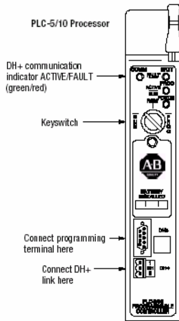
Figure 1.5 The processor of a PLC (Courtesy: Allen-Bradley)
