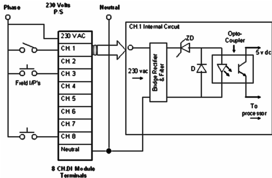
Figure 1.12 Digital AC input module
