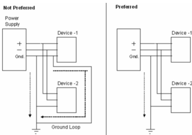
Figure 1.22 Ground loop
