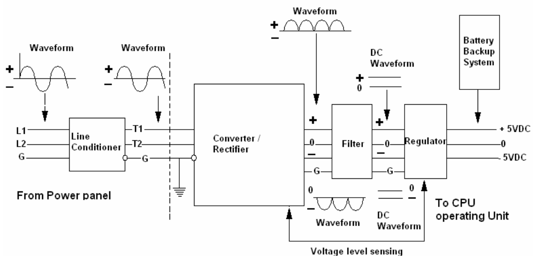
Figure 1.4 Power supply
