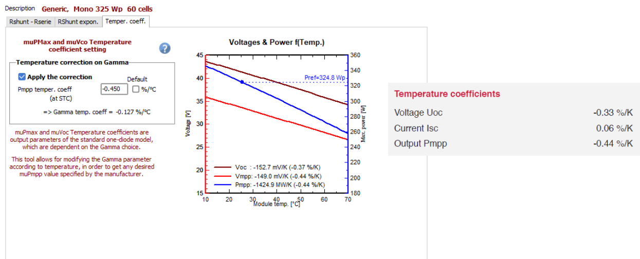
Figure 8: Defining the temperature coefficient from the datasheet.
