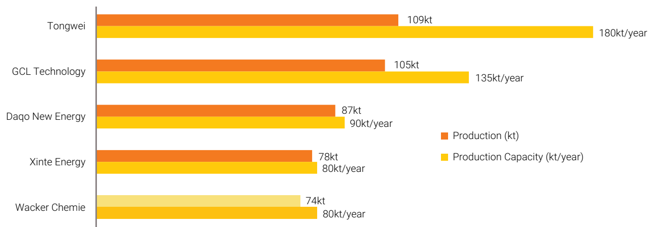
Figure 20 - Manufacturing capacities and production per manufacturer top 5 in 2021
