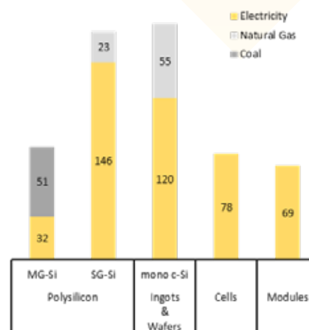
Figure 84- Average energy-intensity [kWh/kWh] per energy vector and per value chain step (Source: IEA) [1]
