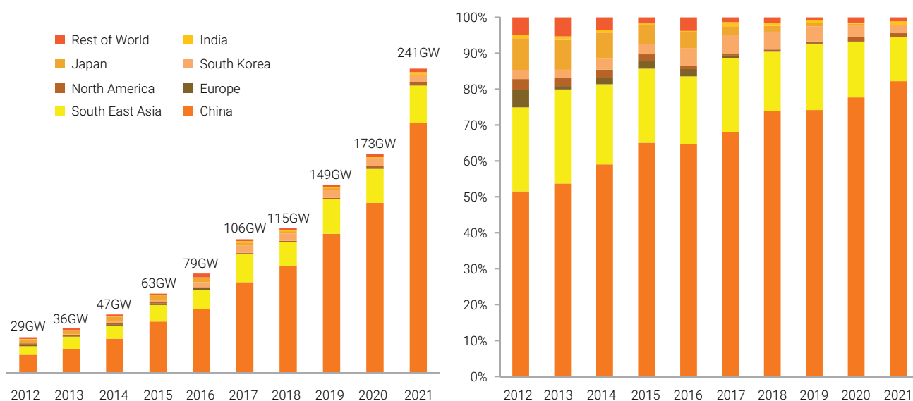
Figure 33 - Evolution of annual cell production per region by capacity (GW) (left) and relative share of the evolution of the cell production per region (right), for the period 2012-2021 (Sources: RTS Corporation)
