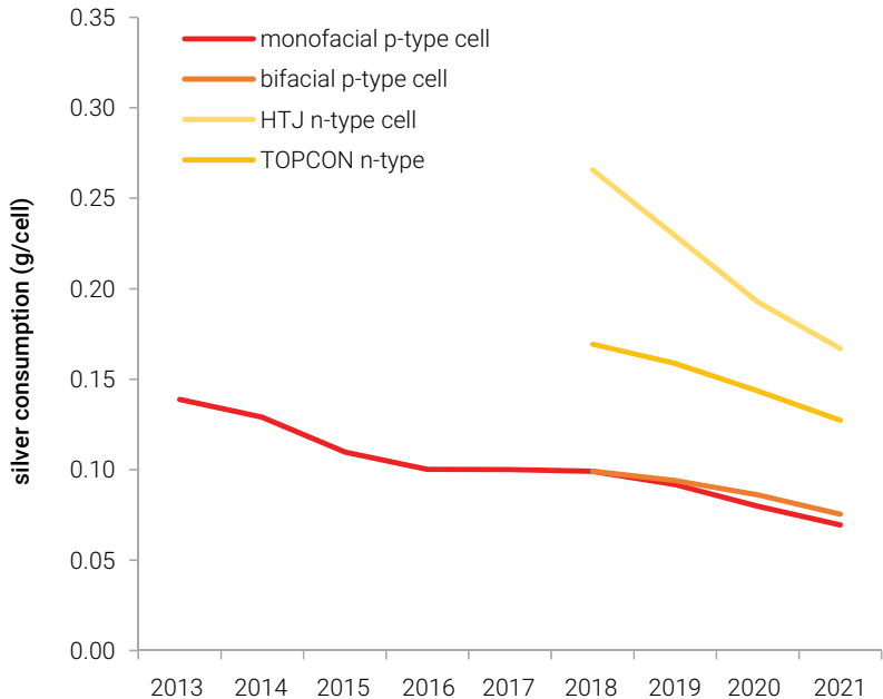
Figure 36 - Evolution of average silver paste consumption per technology for a theoretically assumed constant cell size (M2) (2013-2021) (Sources: ITRPV, Becquerel Institute analysis)
