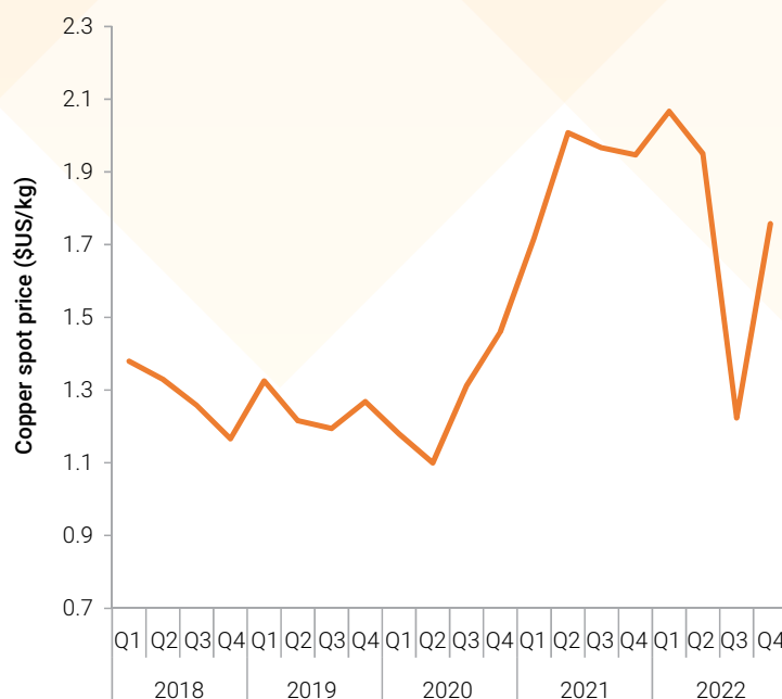
Figure 38 - Quarterly evolution of copper prices (2018-2022) (Sources: tradingeconomics.com)
