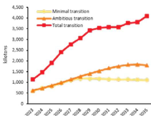
Figure 70- Required annual production of metallurgical-grade silicon for the three solar demand scenarios until 2035 (Sources: Becquerel Institute Research & Analysis)
