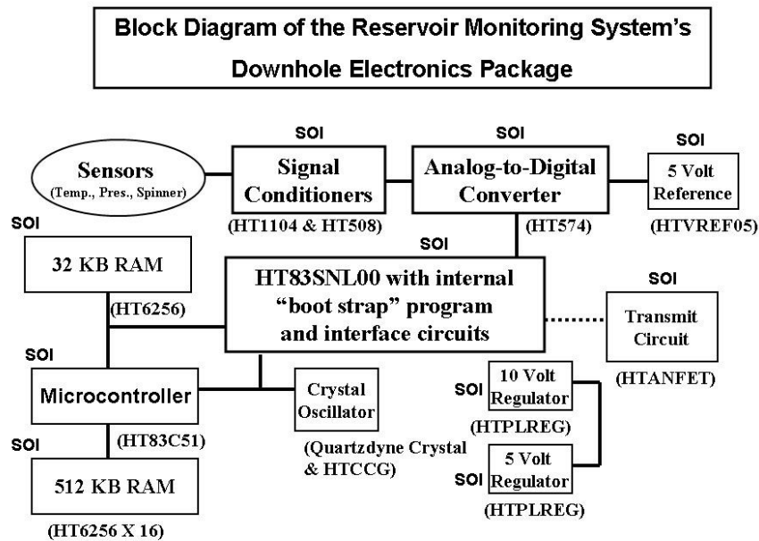
Figure 6-1 Typical downhole tool architecture
