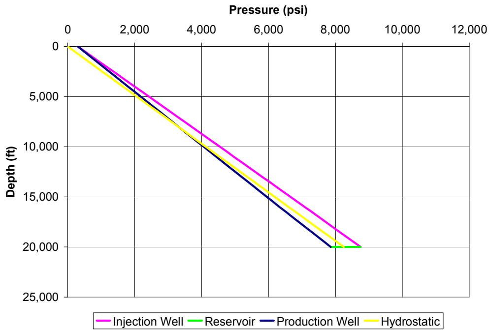
Figure 3-3 Pressure profiles with no ESP
