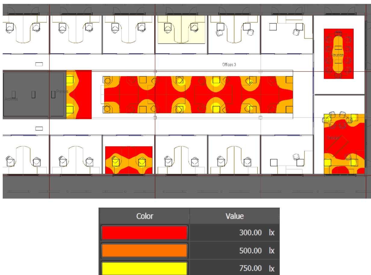
Figure 54. Simulation results for fluorescent lighting on the 80 cm high plane
