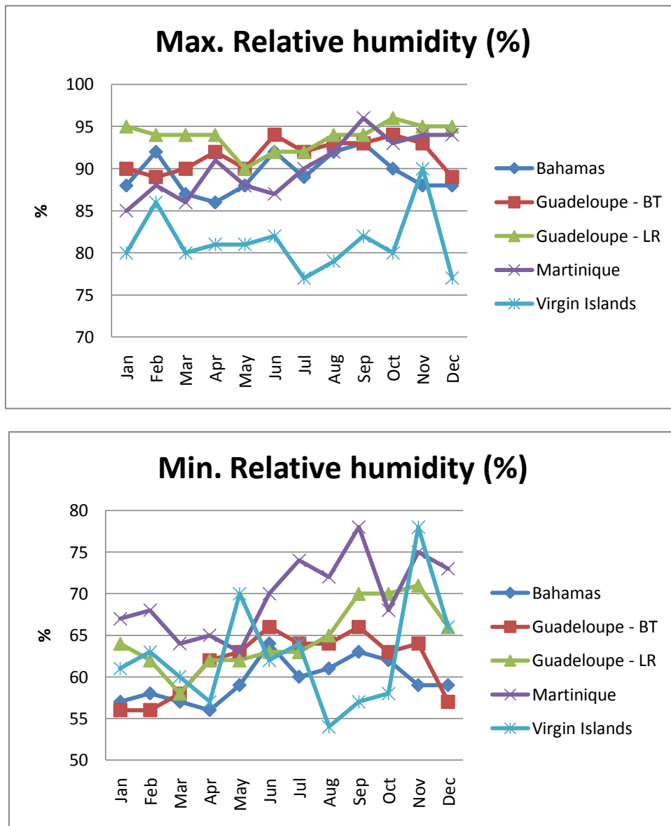
Figure 6. Average monthly relative humidity (%), maximum and minimum; variation throughout the year, for the different stations
