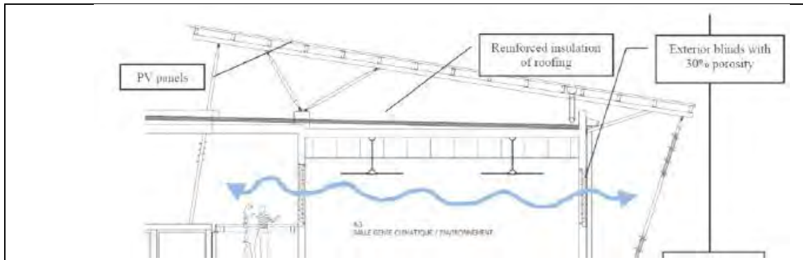
Figure 81- Detail of the roof
