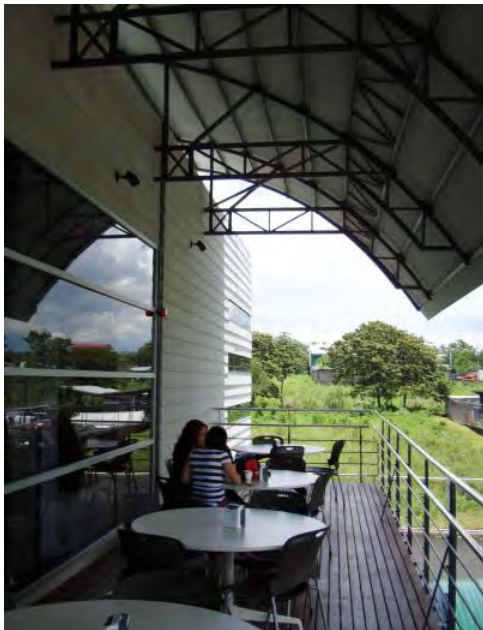
Figure 11- Some constructive elements can be designed to provide solar protection on roofs and façades, protection from the rain and creation of transition spaces (left); protection devices may be fixed or mobile and adapted to the different conditions depending on the orientation
