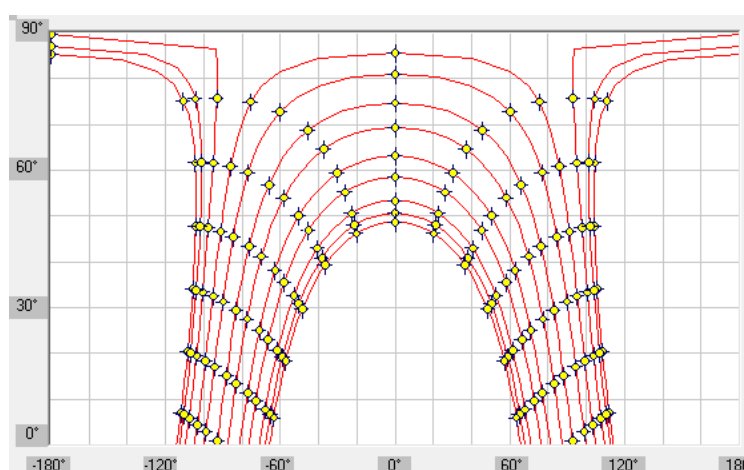
Figure 9- Façades are designed in a different way according to their orientation (left); depending on the latitude the sun path changes is different and thus the incidence on facades and roofs varies. For an average latitude in the Caribbean, the central months of the year represent a considerable incidence on the North façade, as shown by the orthographic projection (right)
