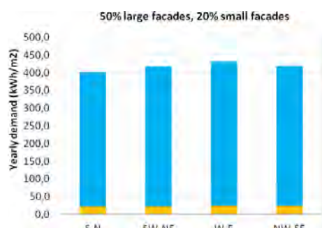
Figure 32- Yearly demand for 50% glazing on large facades and 20% glazing on small facades
