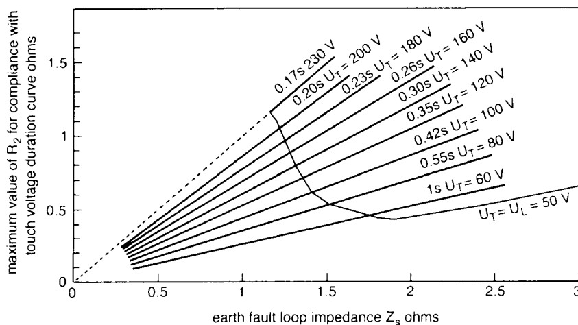
Figure A.12 Impedance characteristic and superimposed touch voltage lines.
