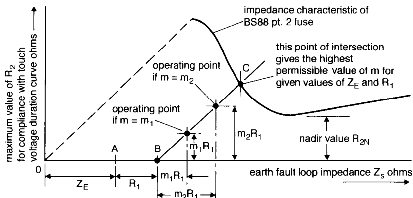
Figure A.11 Using impedance characteristic to determine maximum tolerable value of m .
