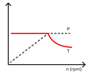
Figure 5.4. Typical torque and power curves in a constant power/torque application.
