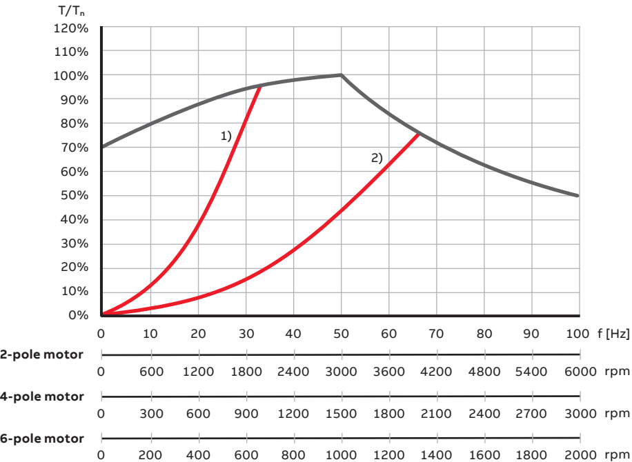
Figure 7.1 Motor loadability curves in a pump and fan application. Comparison of 1) 2-pole and 2) 4-pole motors.
