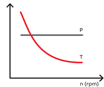
Figure 5.3. Typical torque and power curves in a constant power application.
