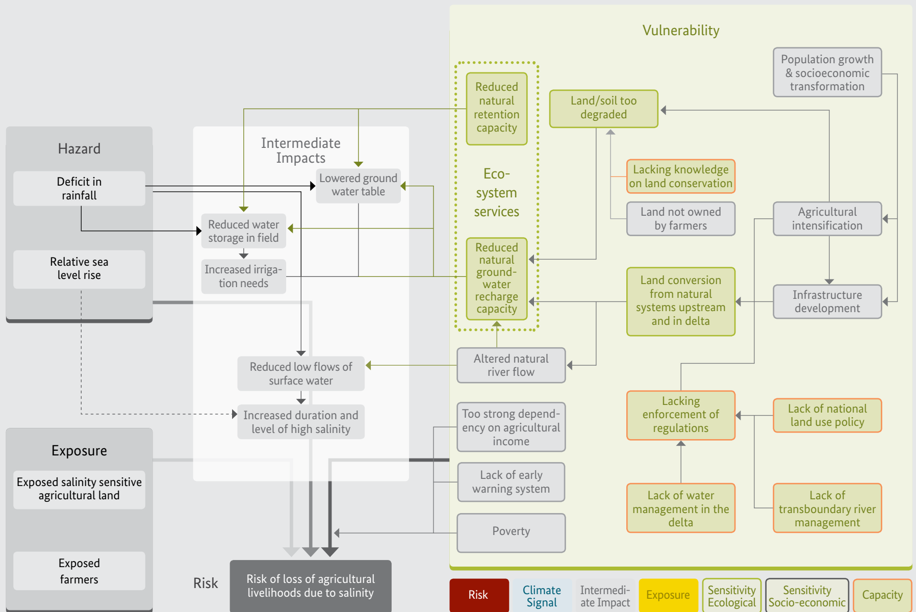
Figure_Anx 6: Entry points for adaptation practitioners and planners working on natural resource conservation and management (green coloured boxes)
