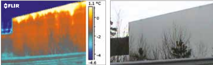
A warehouse with a lot of warm air escaping between the wall and the roof. These joints should be tightened to stop the energy loss.
