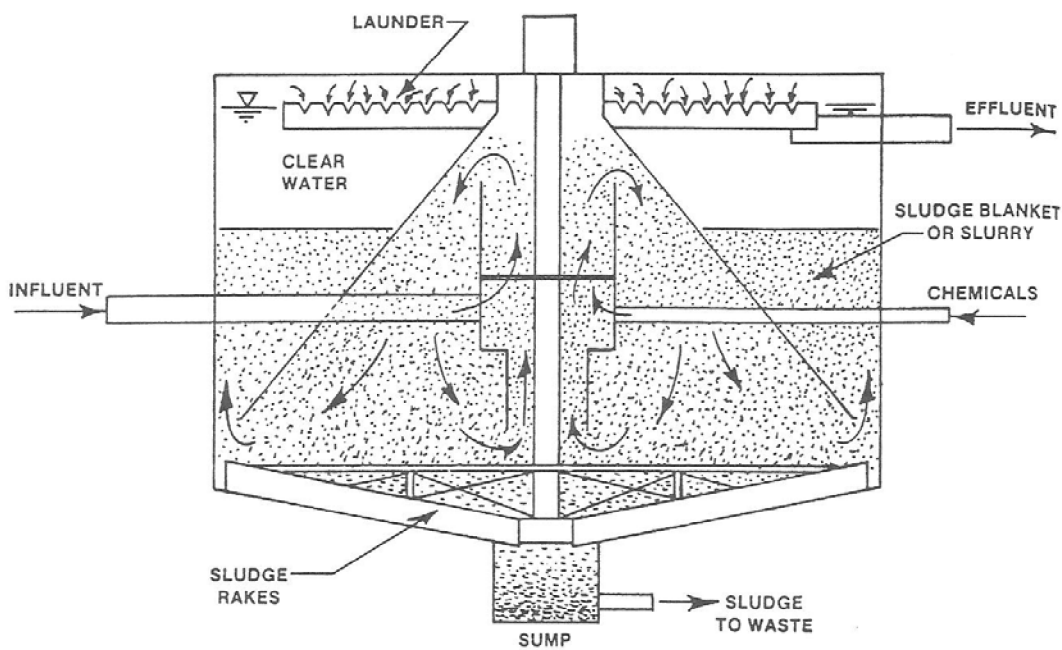
Solids-contact unit
