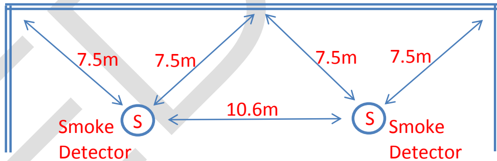
Distance between Smoke Detectors
