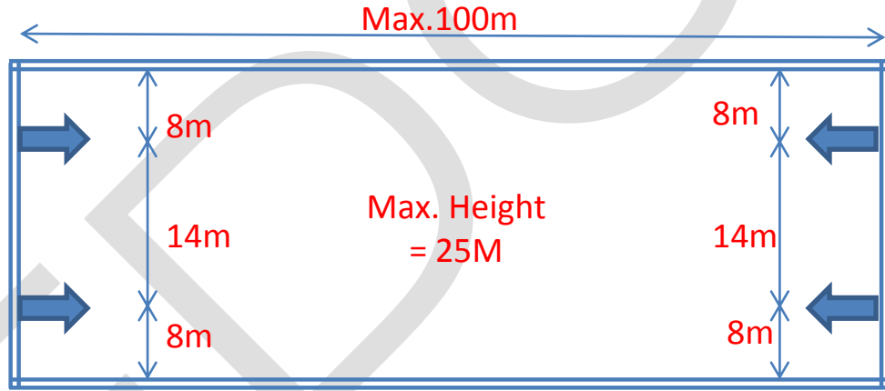
Distance between Beam Detectors
