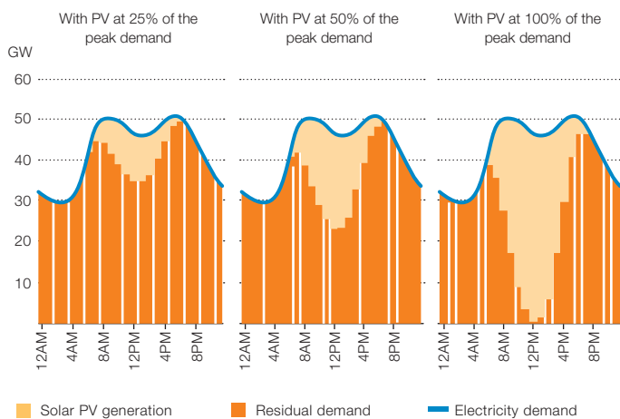
Indicative daily electricity demand and residual demand with expanding deployment of solar PV (Source: IEA, World Energy Outlook 2013)
