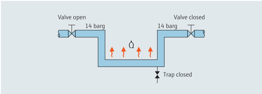
Figure 16: Column close water hammer, starting condition.
