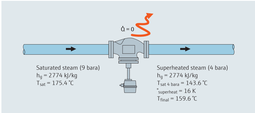
Figure 14: The passage of steam under isenthalpic conditions through a pressure reducing valve (PRV) for known conditions.
