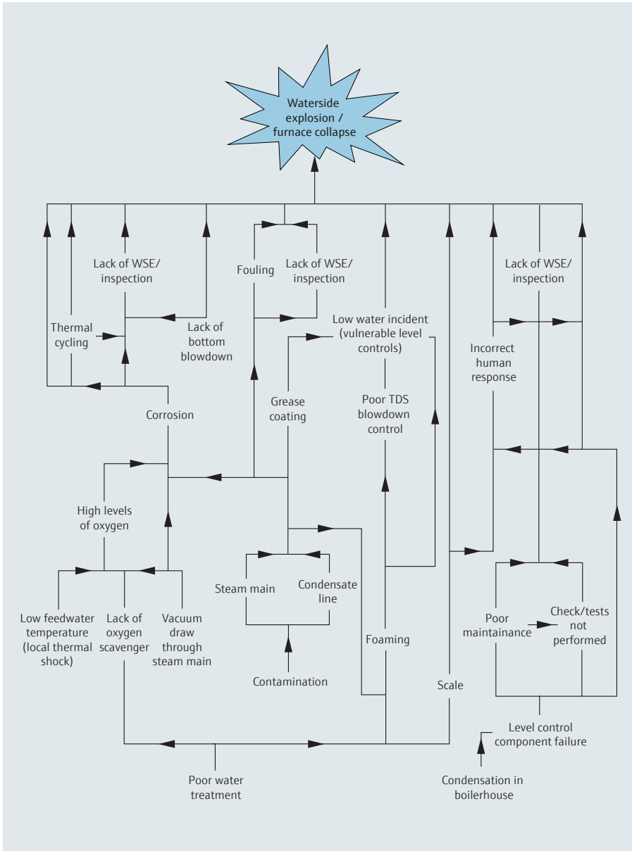
Figure 24: Causal factors of a waterside explosion or furnace collapse for MTHS boilers (although the diagram is based on actual historical accidents, it is not exhaustive). WSE = Written Schemes of Examination.
