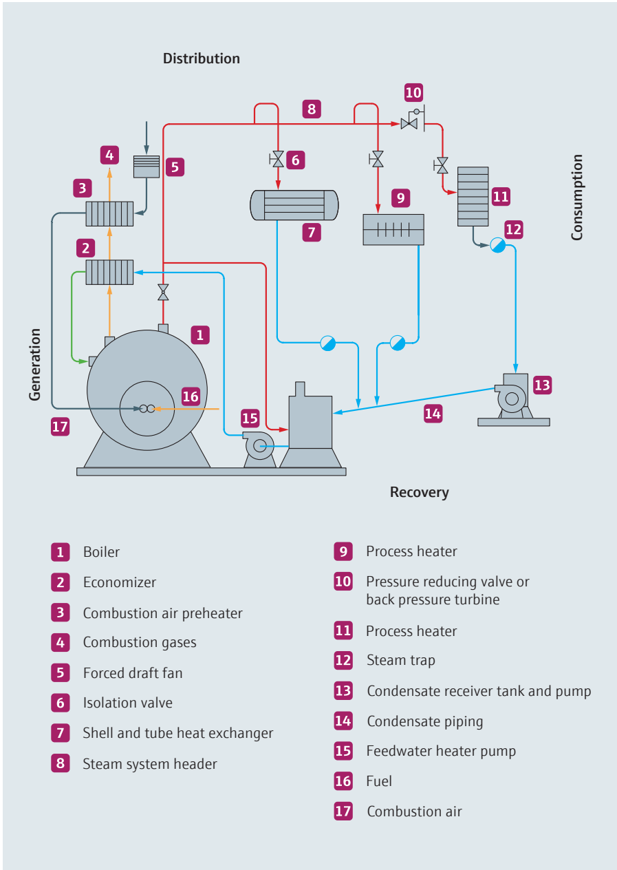
Figure 11: Components of a steam generation and distribution system.
