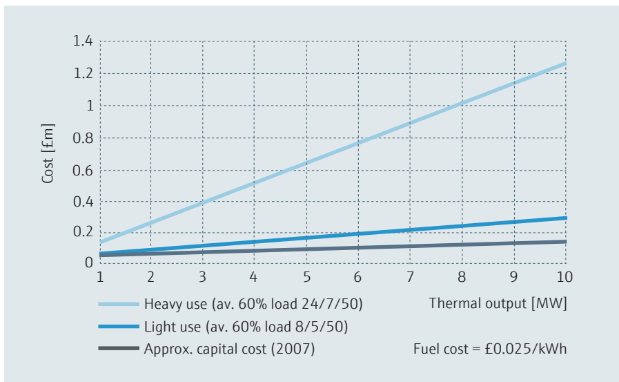
Figure 31: Fuel versus capital costs of industrial boilers.
