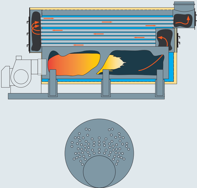
Figure 9: Cutaway of a three-pass wetback MTHS boiler.
