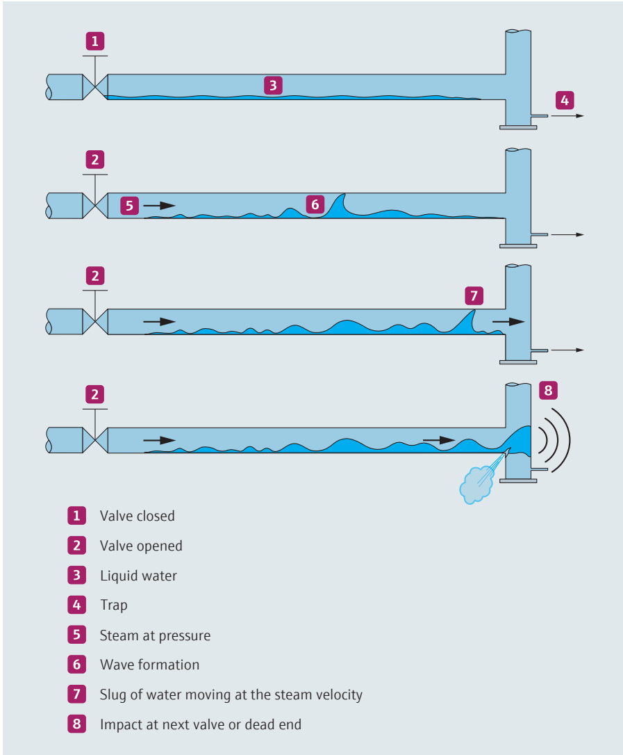
Figure 22: An example of plug flow water hammer.
