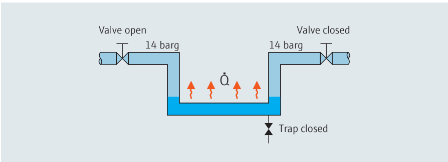
Figure 17: Column closure water hammer, stratification and sub-cooling.
