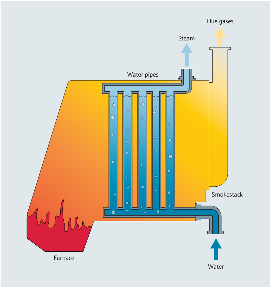
Figure 5: Principle of a water-tube boiler.
