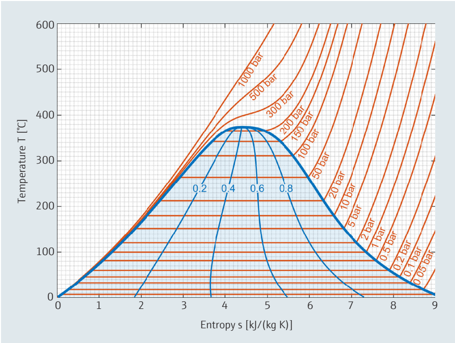
Figure 33: Mollier diagram (blue curves = dryness fraction).
