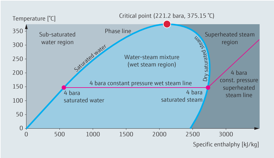
Figure 34: Simplified T-h phase diagram (Mollier diagram) with a 4 bar constant pressure line.
