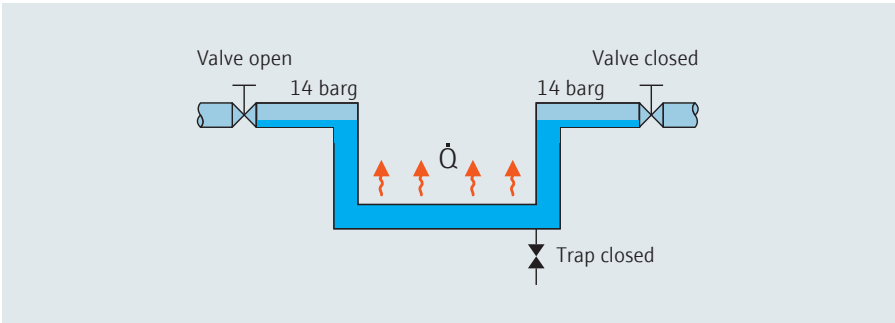
Figure 18: Column closure water hammer, flooding and steam pocket collapse.
