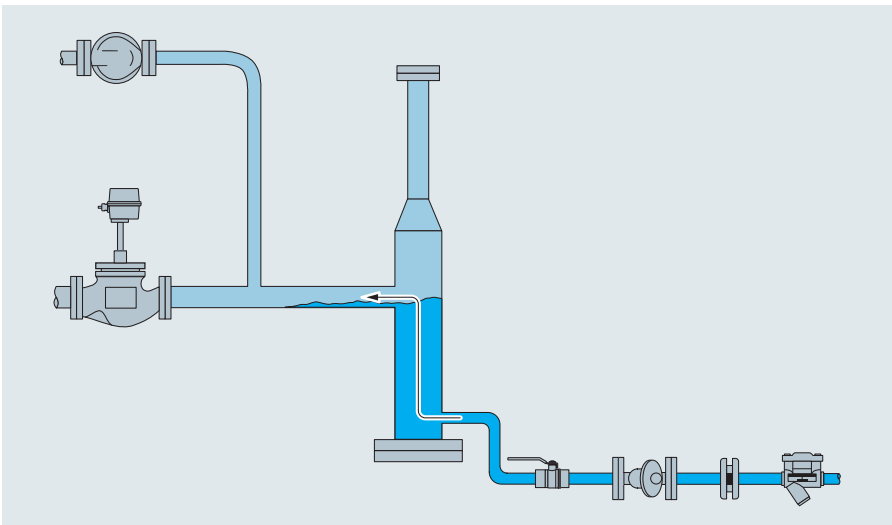
Figure 21: Condensate collection due to trap failing closed.
