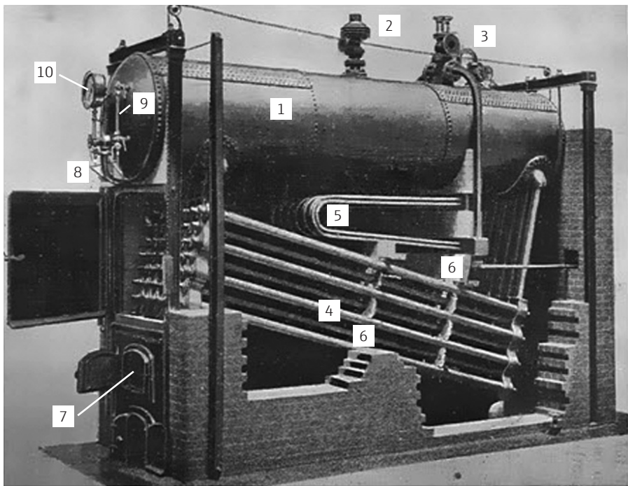
Figure 6: A Babcock and Wilcox water-tube boiler. From: Ripper, William C.H. (1923). Heat Engines , London, p. 207.
