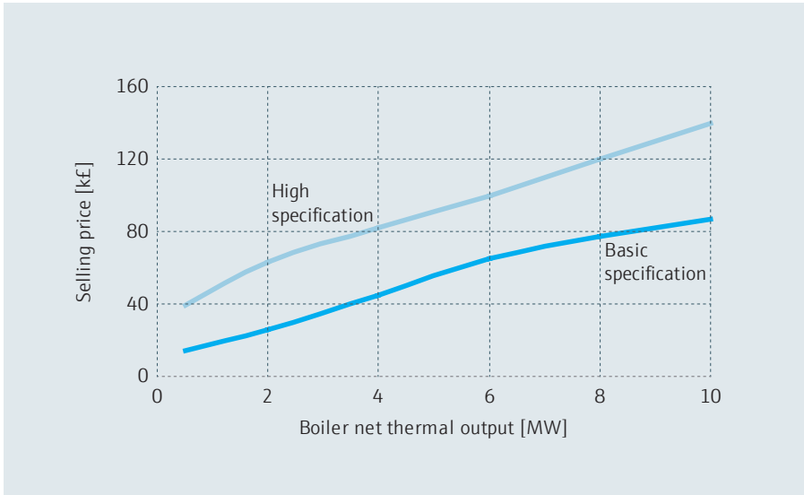
Figure 32: MTHS boiler cost variation (for 2007) due to specification enhancement.
