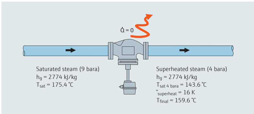
Figure 12: The passage of steam under isenthalpic conditions through a pressure reducing valve (PRV) for known conditions.
