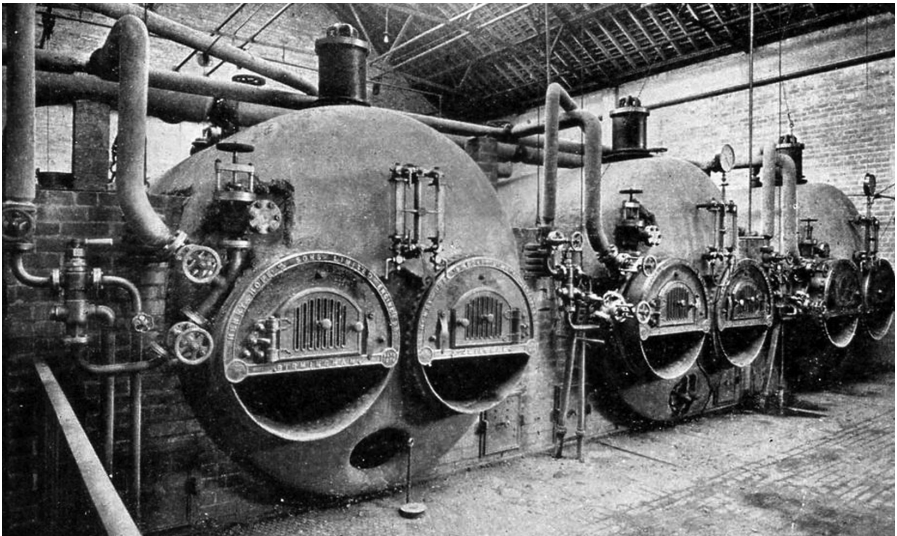
Figure 2: Boiler house with three Lancashire boilers (second half 19th century). Source: Heritage group of the CIBSE ( www.hevac-heritage.org ).
