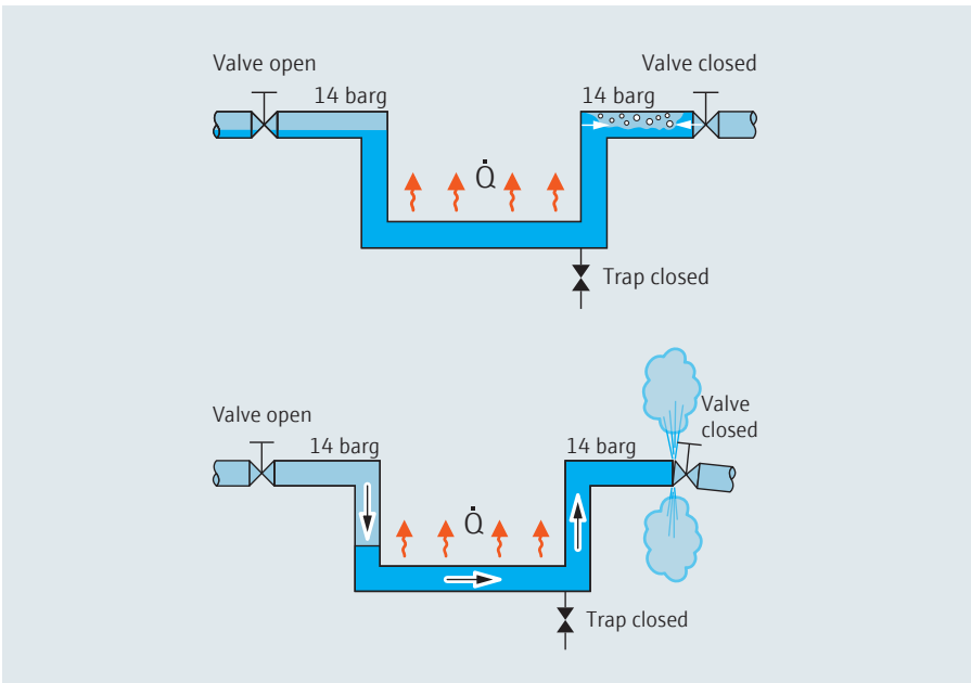
Figure 19: Column closure water hammer, line rupture.
