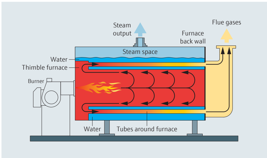
Figure 10: Cutaway of a reverse flame MTHS boiler.
