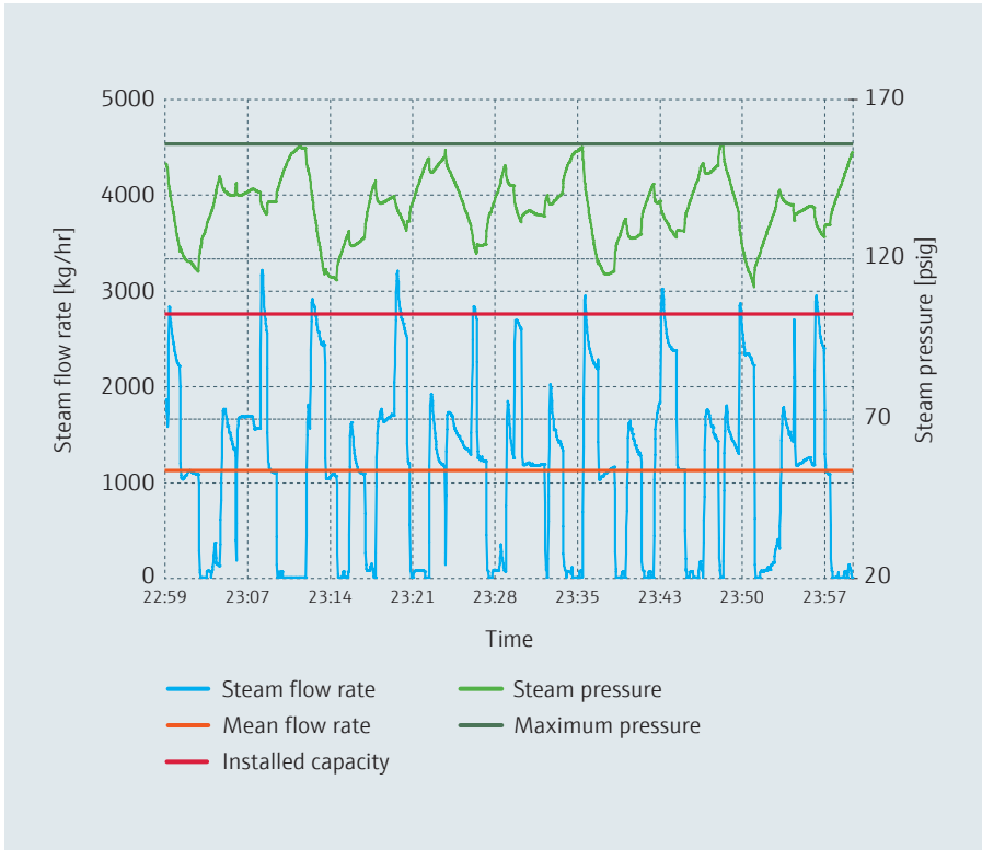
Figure 28: Process data with instantaneous demand profile.
