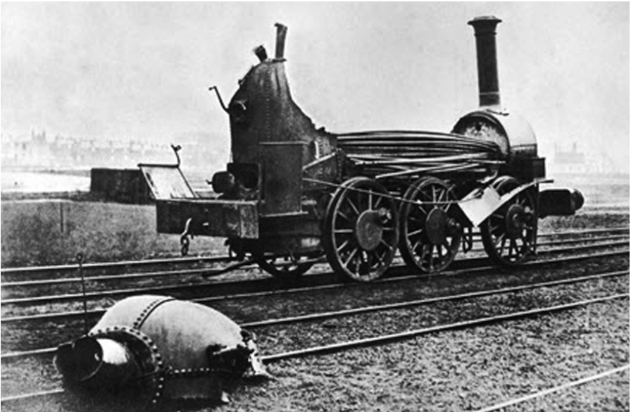
Figure 15: Locomotive boiler explosion and its consequences.
