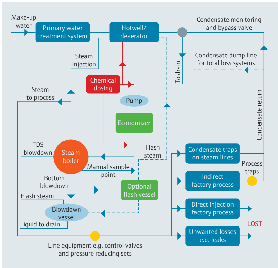
Figure 3: Scheme of a generic steam system.
