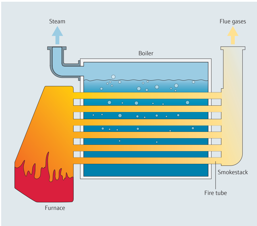
Figure 7: Principle of a fire-tube boiler.
