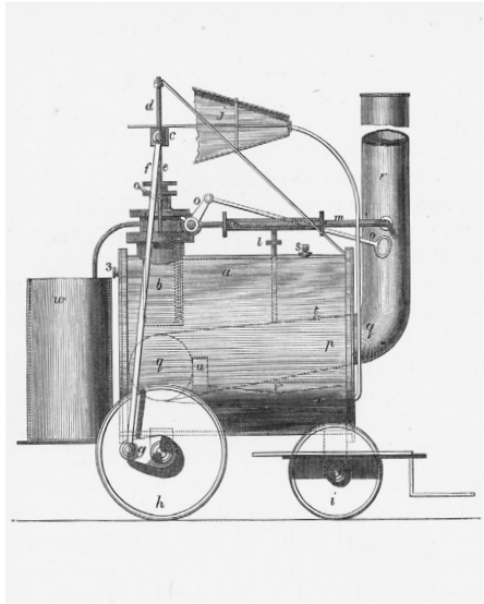
Figure 1: Richard Trevithick (1771–1833). British inventor and mining engineer. Trevithick was the first to successfully use high-pressure steam (then known as “strong” steam). Until ca. 1800, the weakness of existing boilers coupled with the influence of James Watt had generally restricted steam boilers to very low pressures or “weak” steam. Right: Trevithick’s “Puffing Devil” – the first steam-powered locomobile drove on streets, not on tracks.
