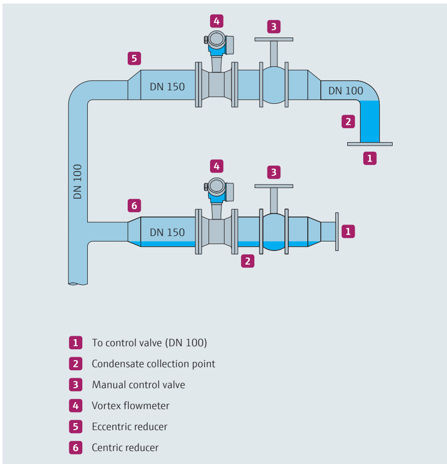
Figure 20: Condensate collection due to trap failing closed.
