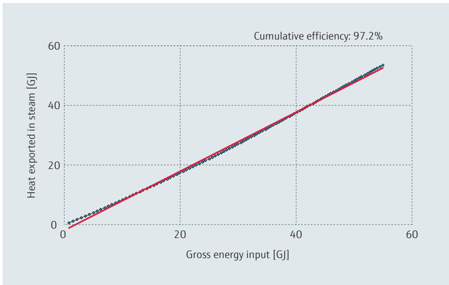
Figure 27: Unrealistic cumulative efficiency data.
