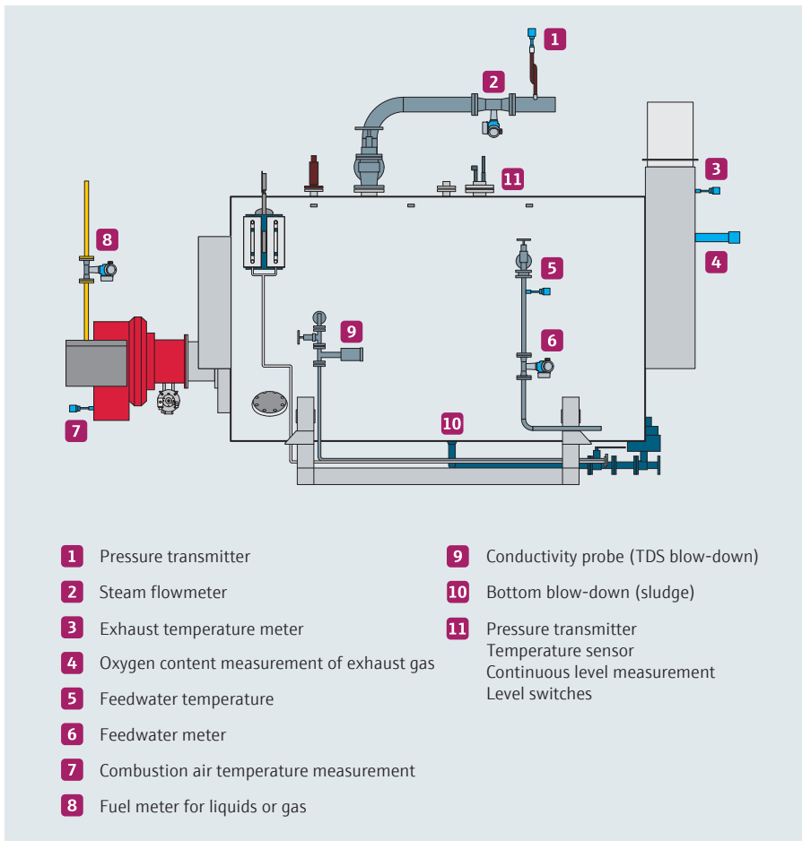
Figure 29: Boiler control with various instruments.
