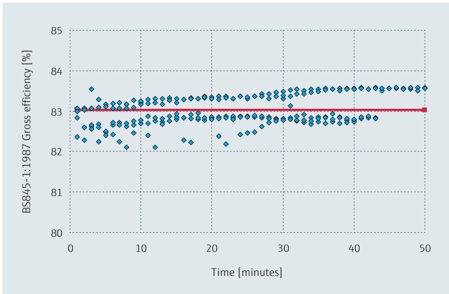
Figure 25: Efficiency measurement according to BS 845-1:1987.
