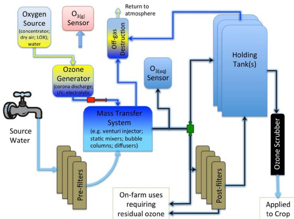
Figure 26. Schematic of ozone disinfection system.
