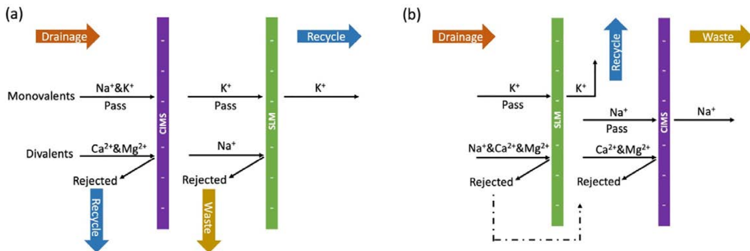
Figure 22. Selective sodium removal via electrodialysis.
