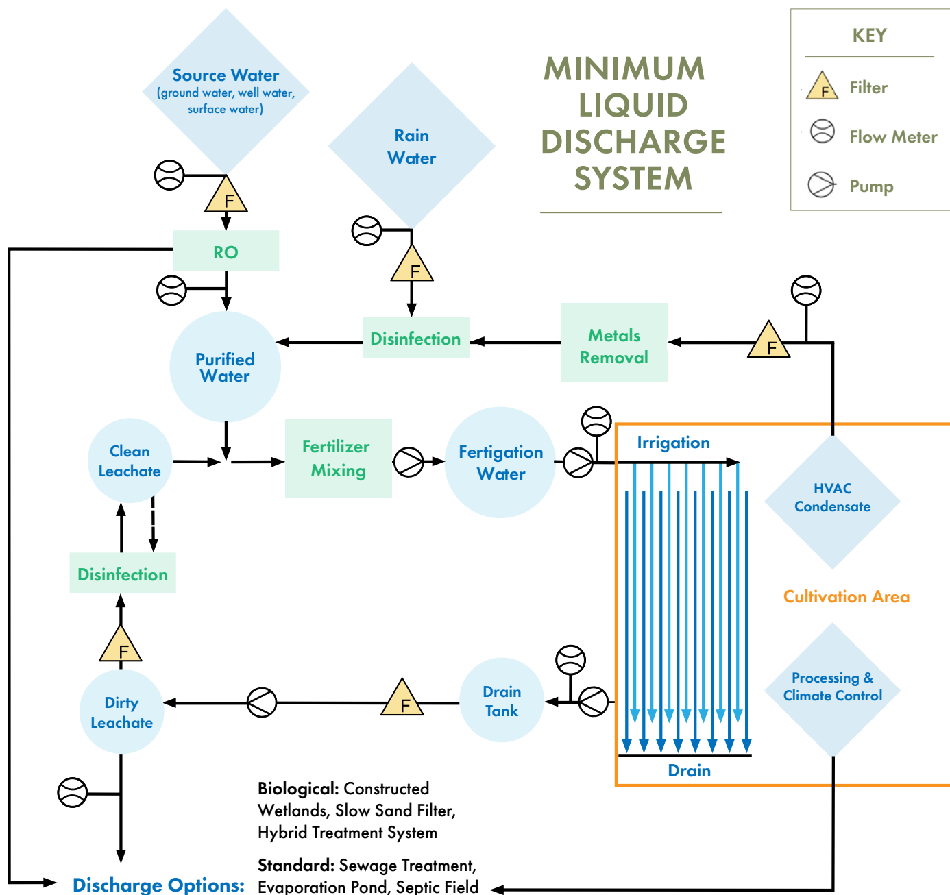
Figure 35. Schematic of a Minimum Liquid Discharge facility with rainwater recapture, condensate recapture, and both standard and biological discharge options. 105
