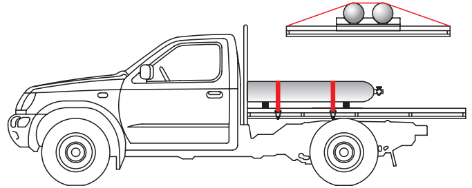
Transporting cylinder lying down. (Note: NEVER transport LPG cylinders, Dissolved Acetylene cylinders or liquefied gas cylinders lying down)
