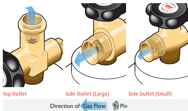
Examining the cylinder valve outlet
