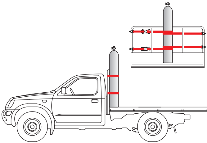
Transporting cylinders upright
