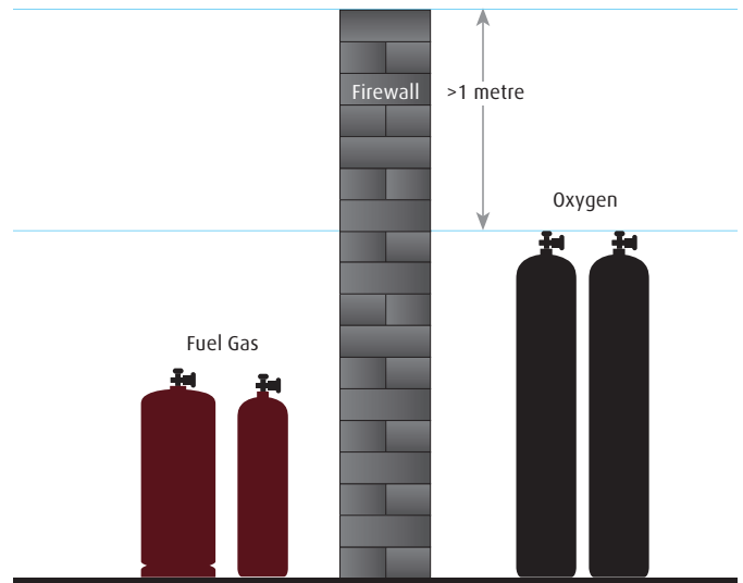
A fire wall must be higher than the tallest cylinder by at least 1 metre
