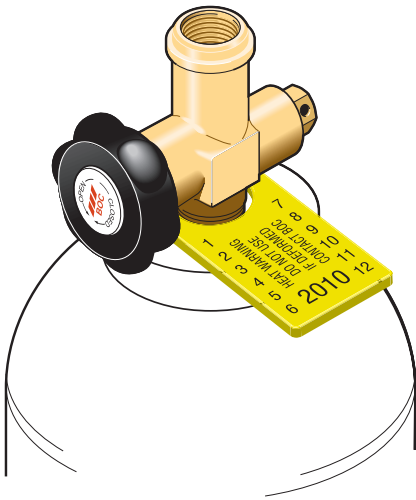
Top outlet valve showing a test date tag
