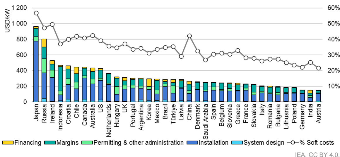
Figure 4.5 Utility-scale solar PV total installed costs vs. share of soft costs, 2021
