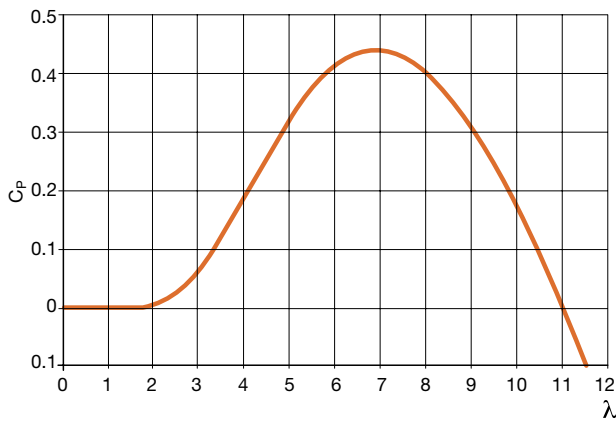
Figure 3.12 - Relation \lambda - C_p ( \beta = 1^\circ )
