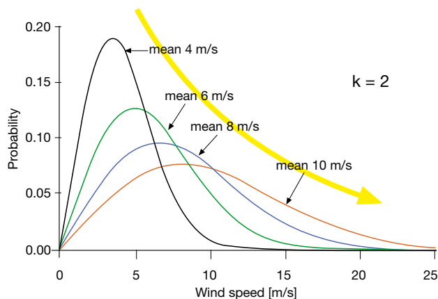
Figure 4.5 - Weibull curve for different mean values of wind speed
