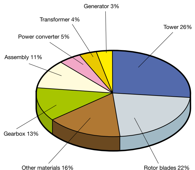
Figure 2.2 - Wind turbine component cost (% of total)
