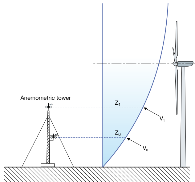
Figure 4.7 - Speed at the hub
