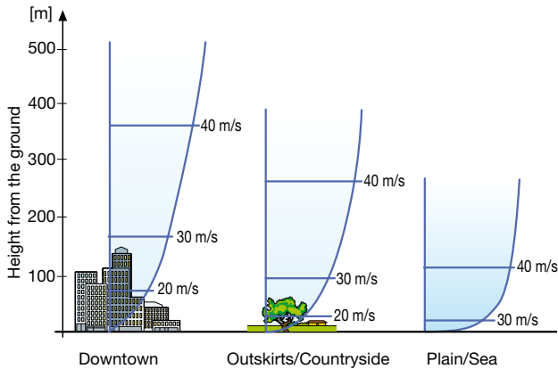
Figure 4.6 - Vertical profile of the wind
