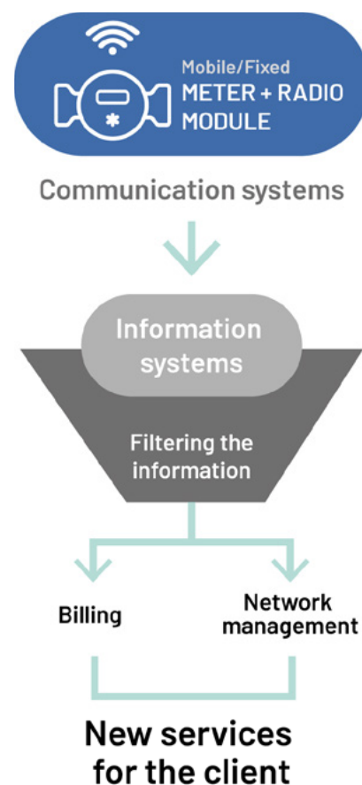
Figure 4.1: Architecture of Consumption Data flow
