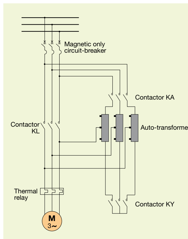
Figure 7: Principle diagram for autotransformer starting
