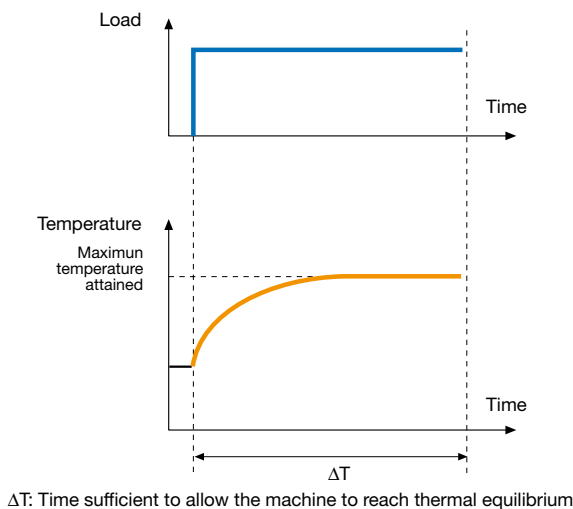
Continuous running duty: Duty type S1
