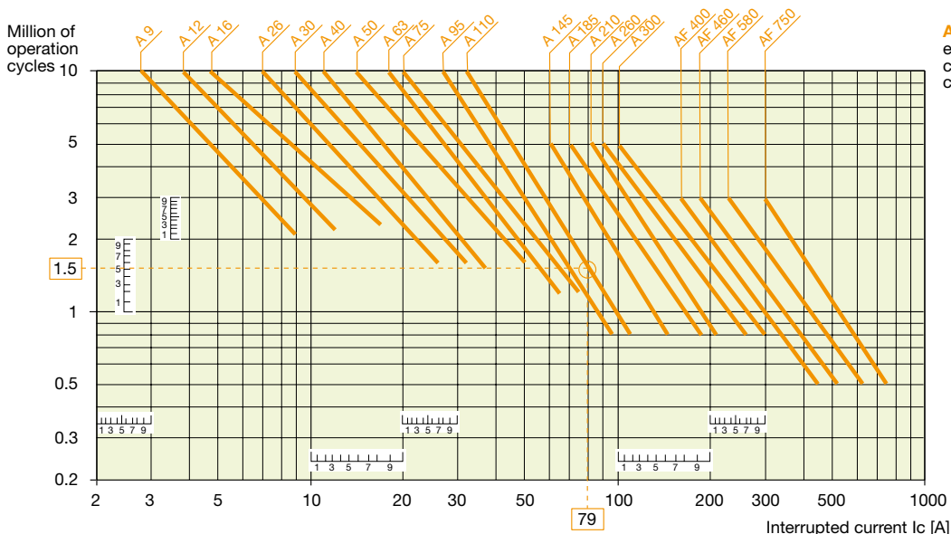
Figure 14: Curves showing the electrical life for the category AC-3 – voltage <440V – ambient temperature <55°C
