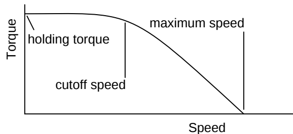
Figure 13.26: Stepper speed characteristics.
