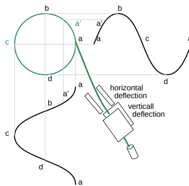
Figure 13.54: X-axis sine and Y-axis cosine trace circle.
