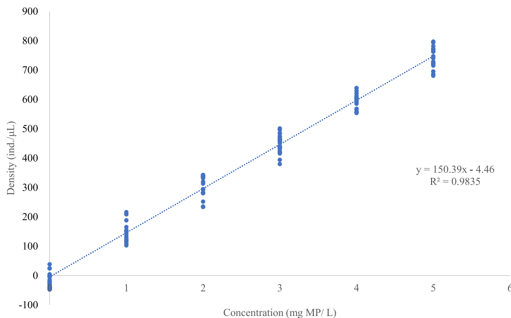
Fig. 4. External calibration curve with presence of matrix showing the relation between signal density and concentration of all study MPs (10, 50, 100 µm), and compositions (PA, PET, PP, PS, PVC). The sample matrix was Reagent's Park water and included 2% methanol.
