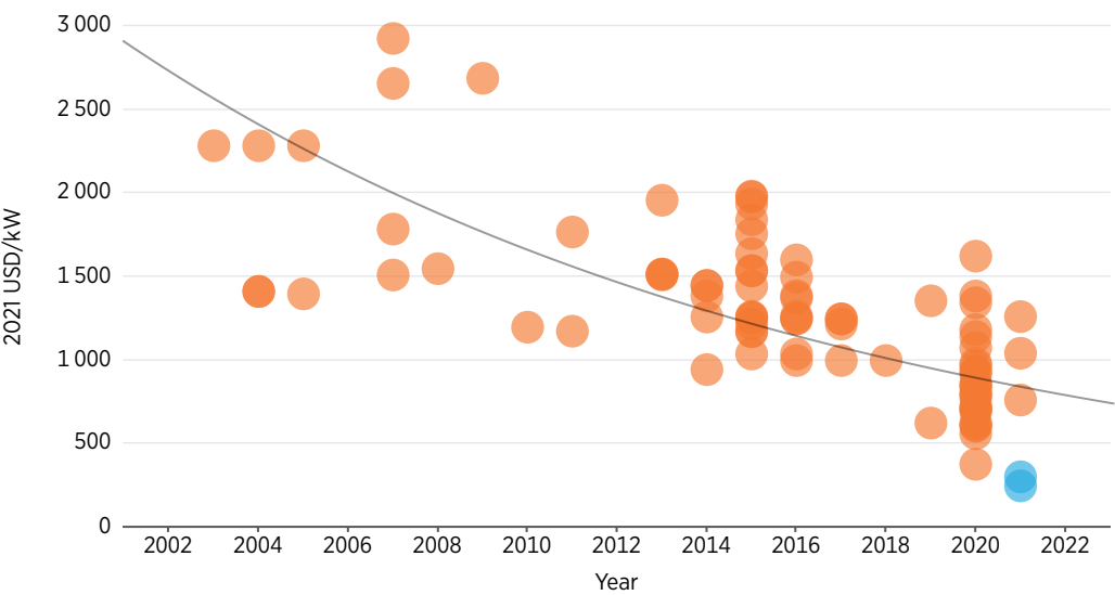
Figure 1.9 Cost trends for alkaline electrolysers, 2003-2021
