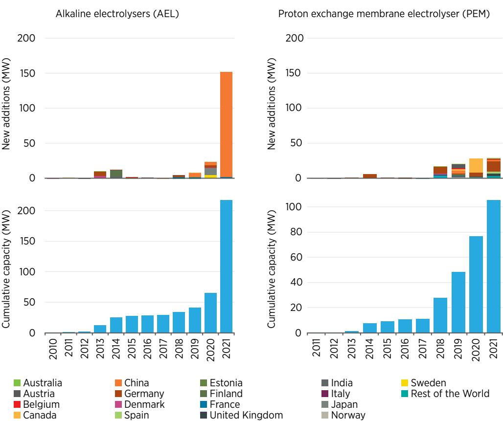
Figure 1.19 Global cumulative capacity in hydrogen electrolyzers, 2010-2021
