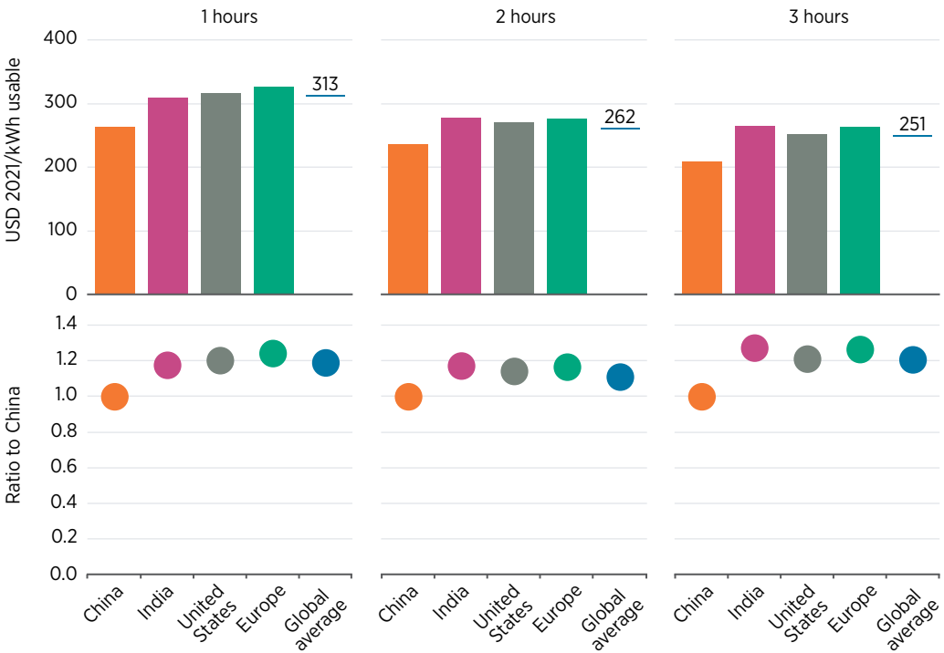
Figure 1.13 Turnkey battery storage system prices by market and duration, 2021
