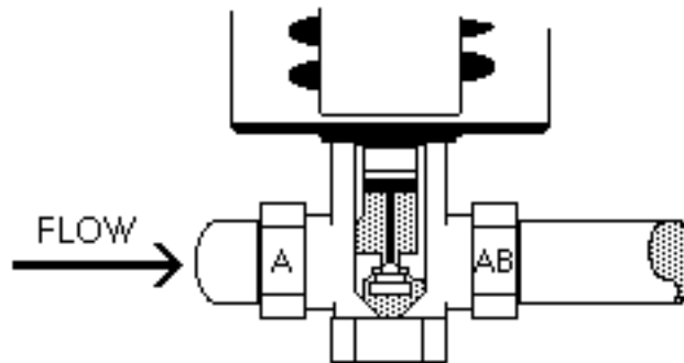
Normally Closed Valve
